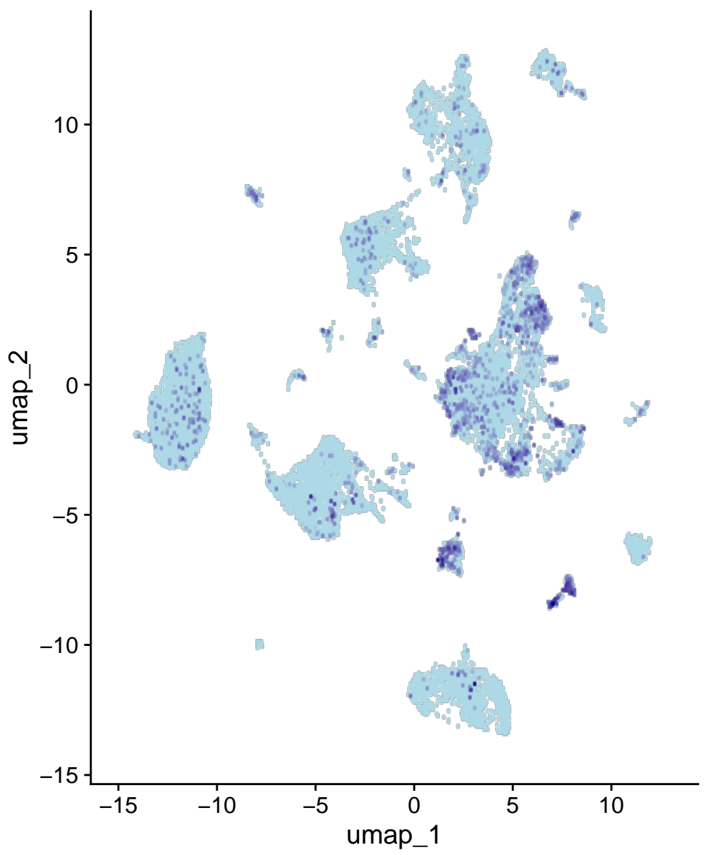
Slc12a8
