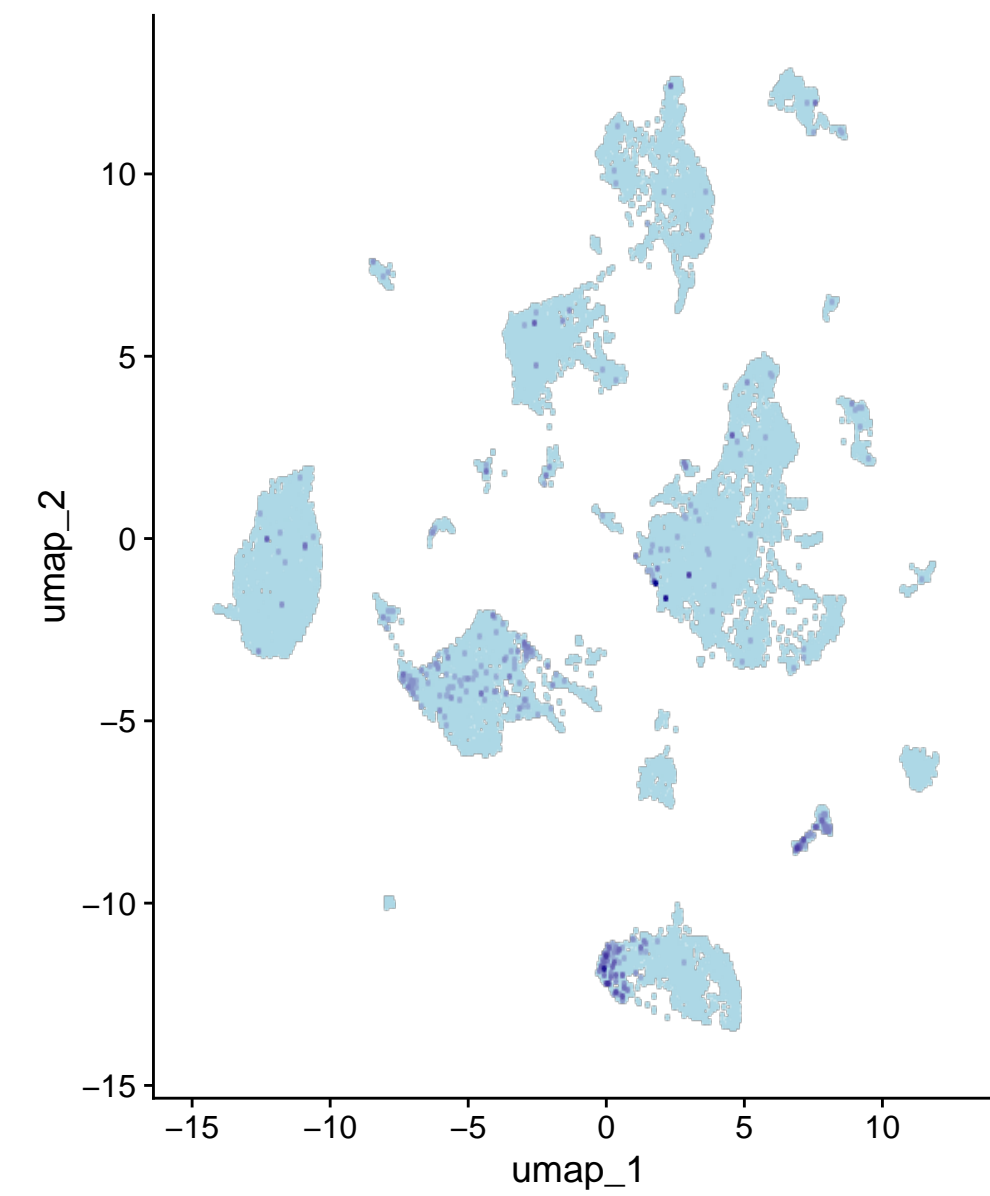
Fn1
