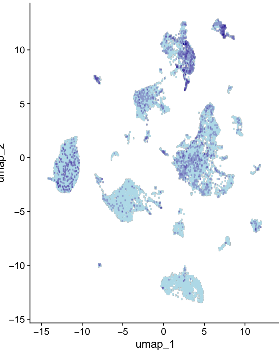
Antxr1
