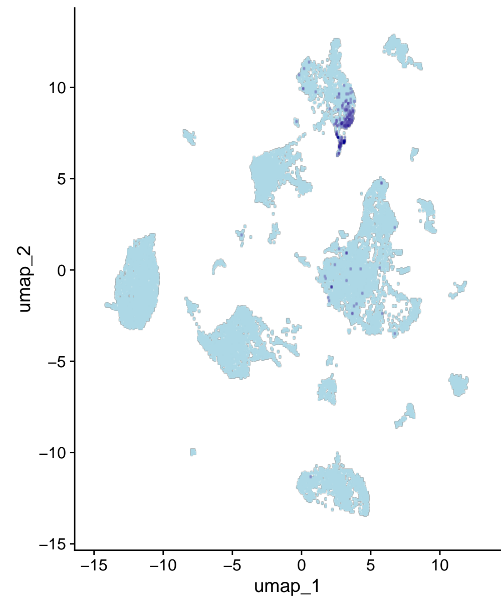
Abi3bp
