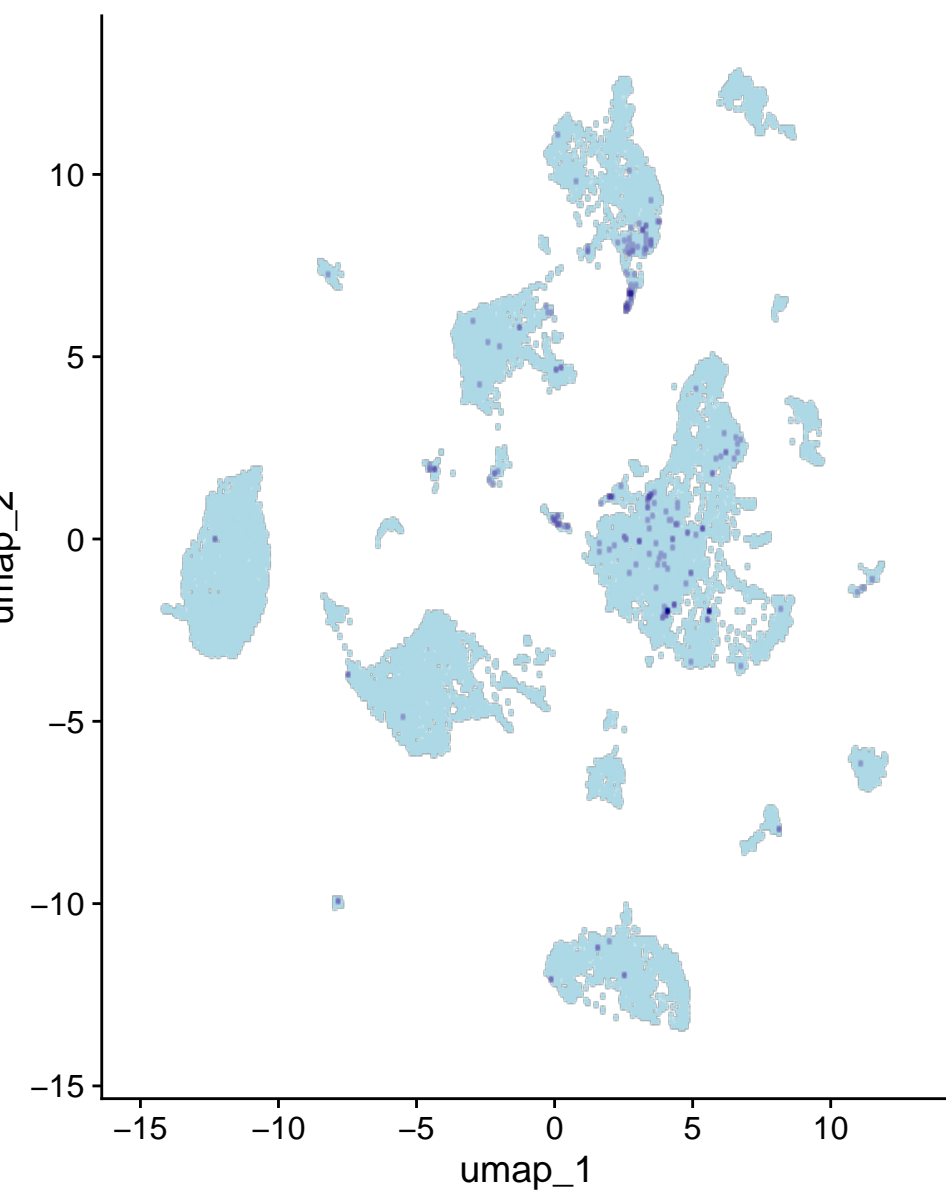
Pdznr3
