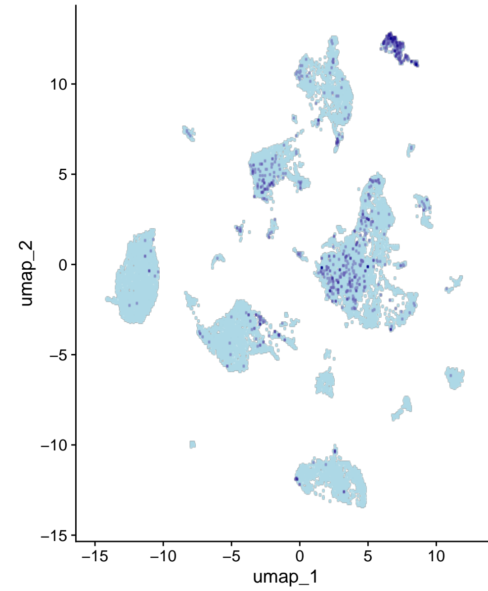
9130024F11Rik
