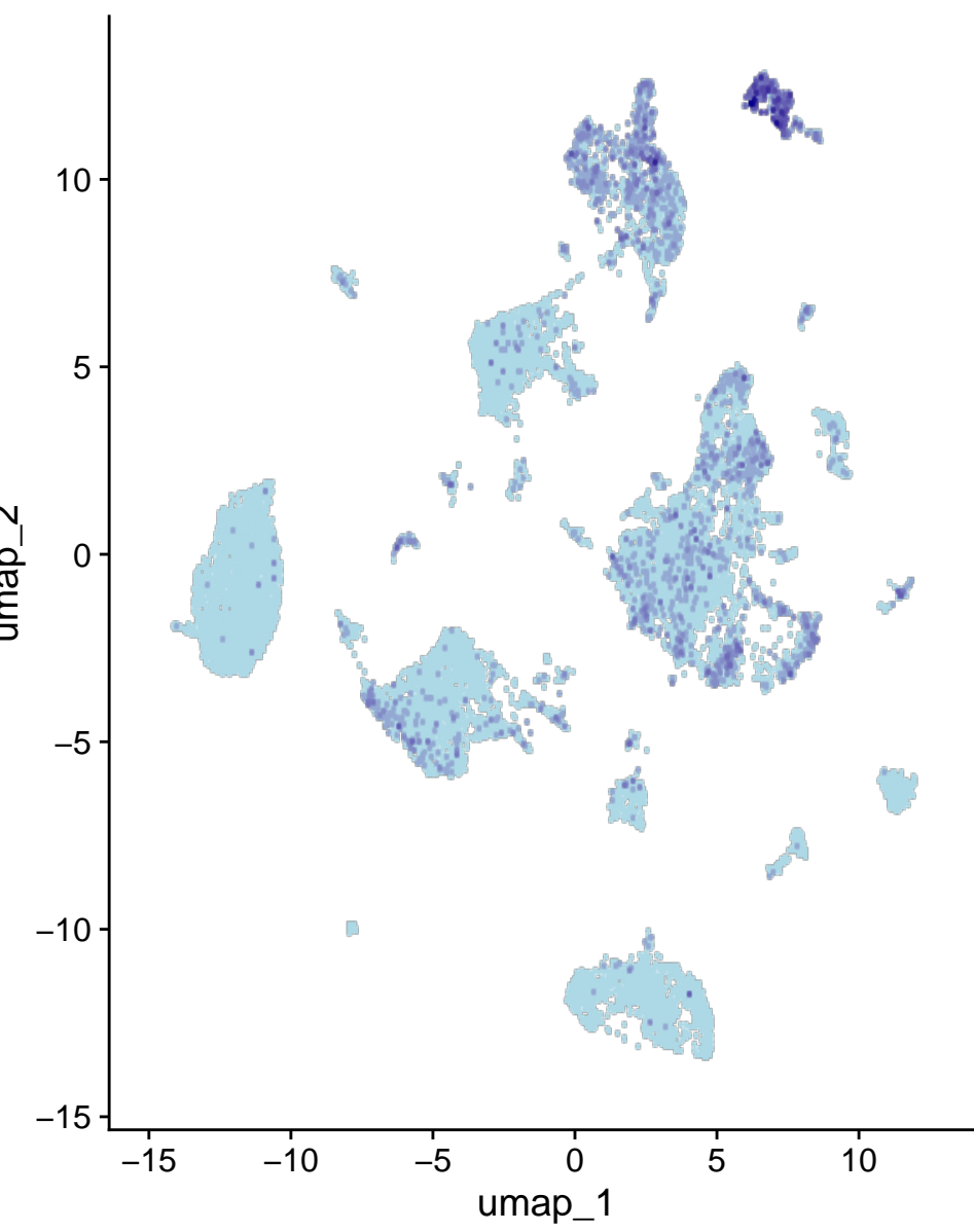
Slc17a7
