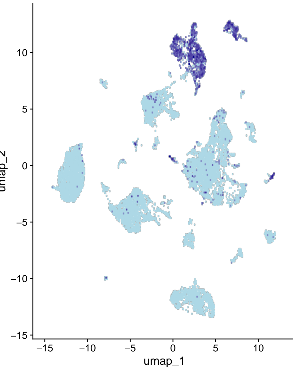
Myocd
