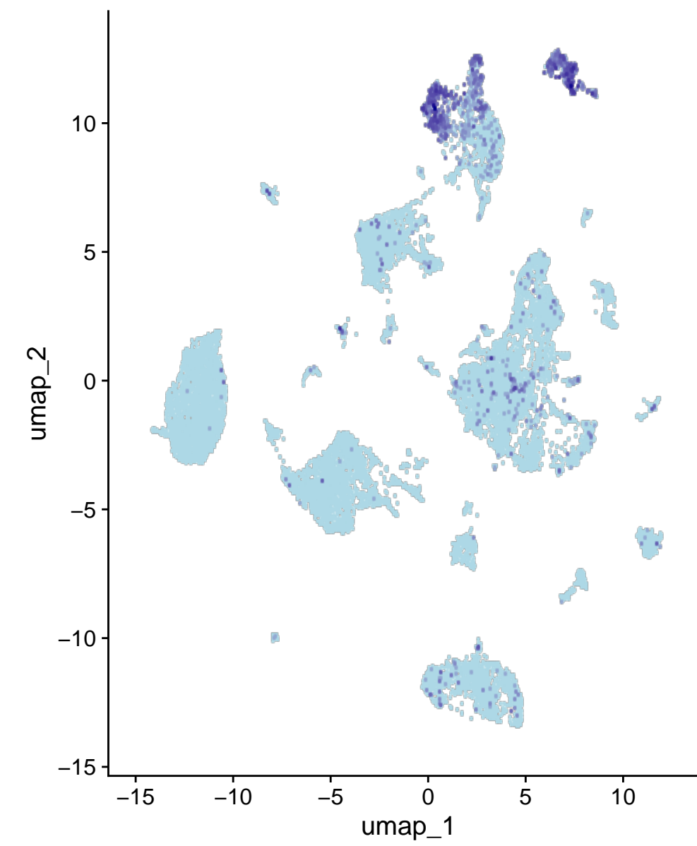
Col12a1
