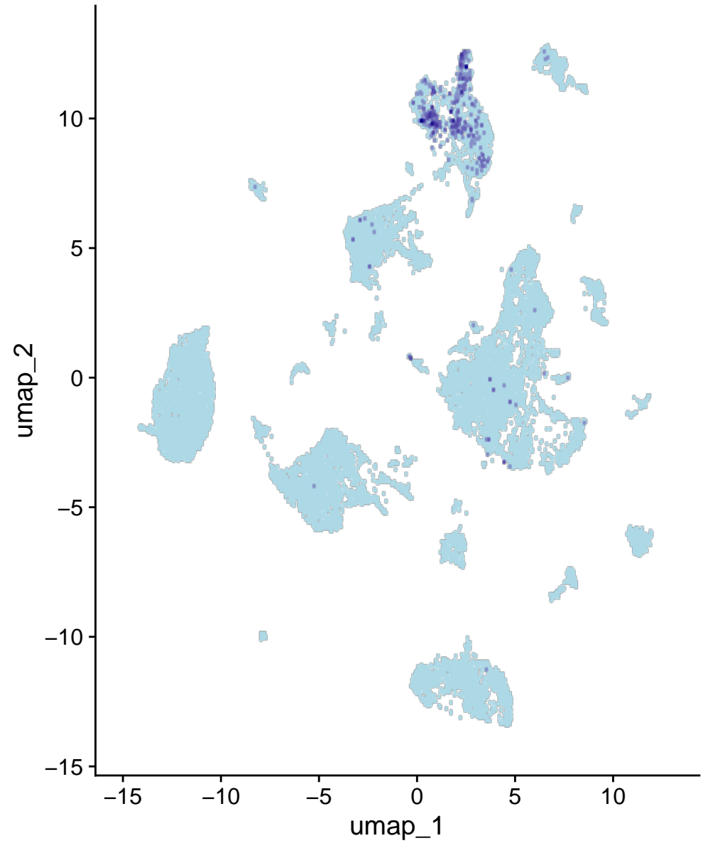
Satb2
