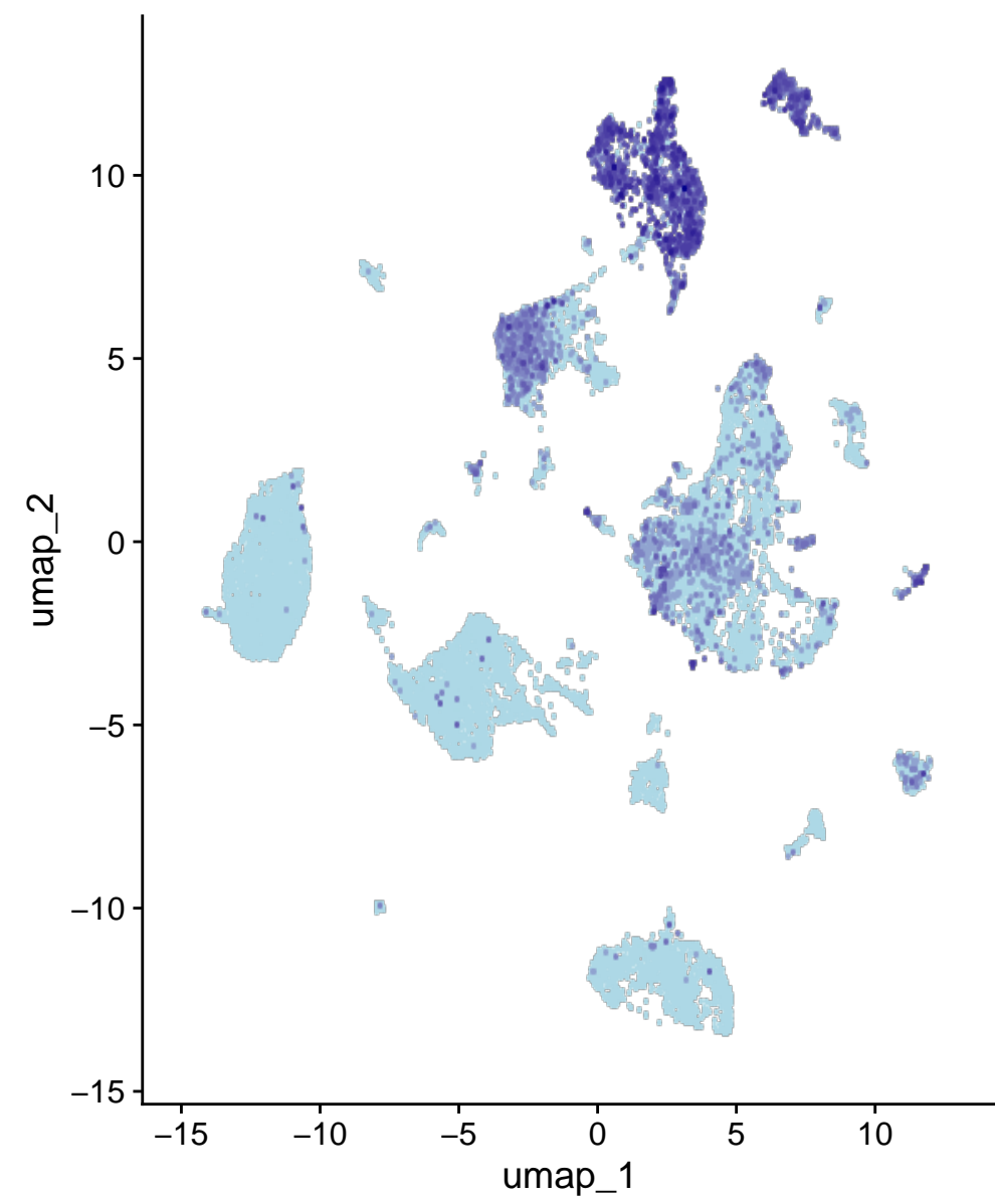
Gm19410
