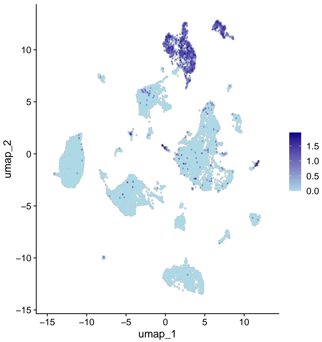
Neurod2
