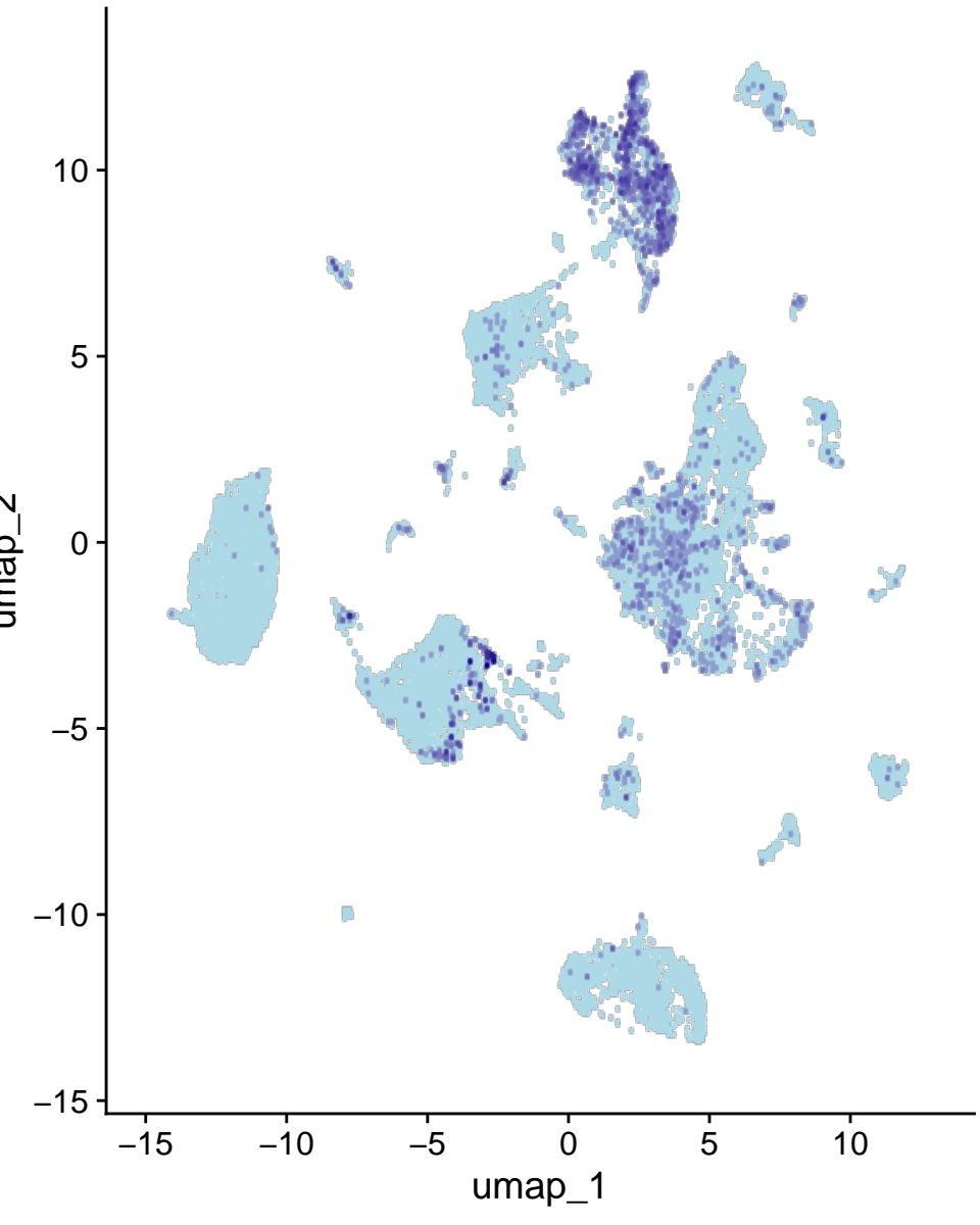
Rtn4r
