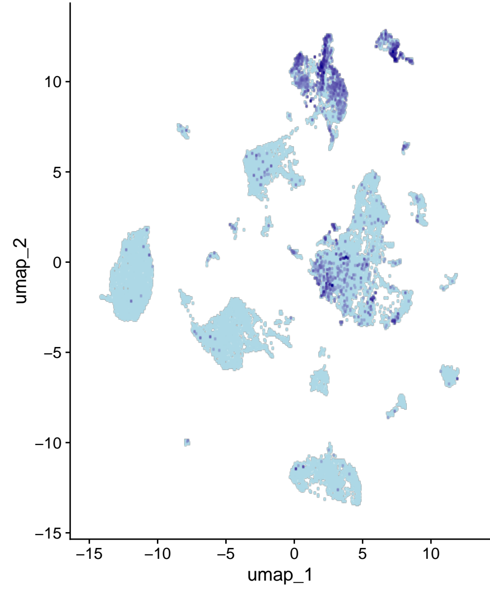
Gm49678
