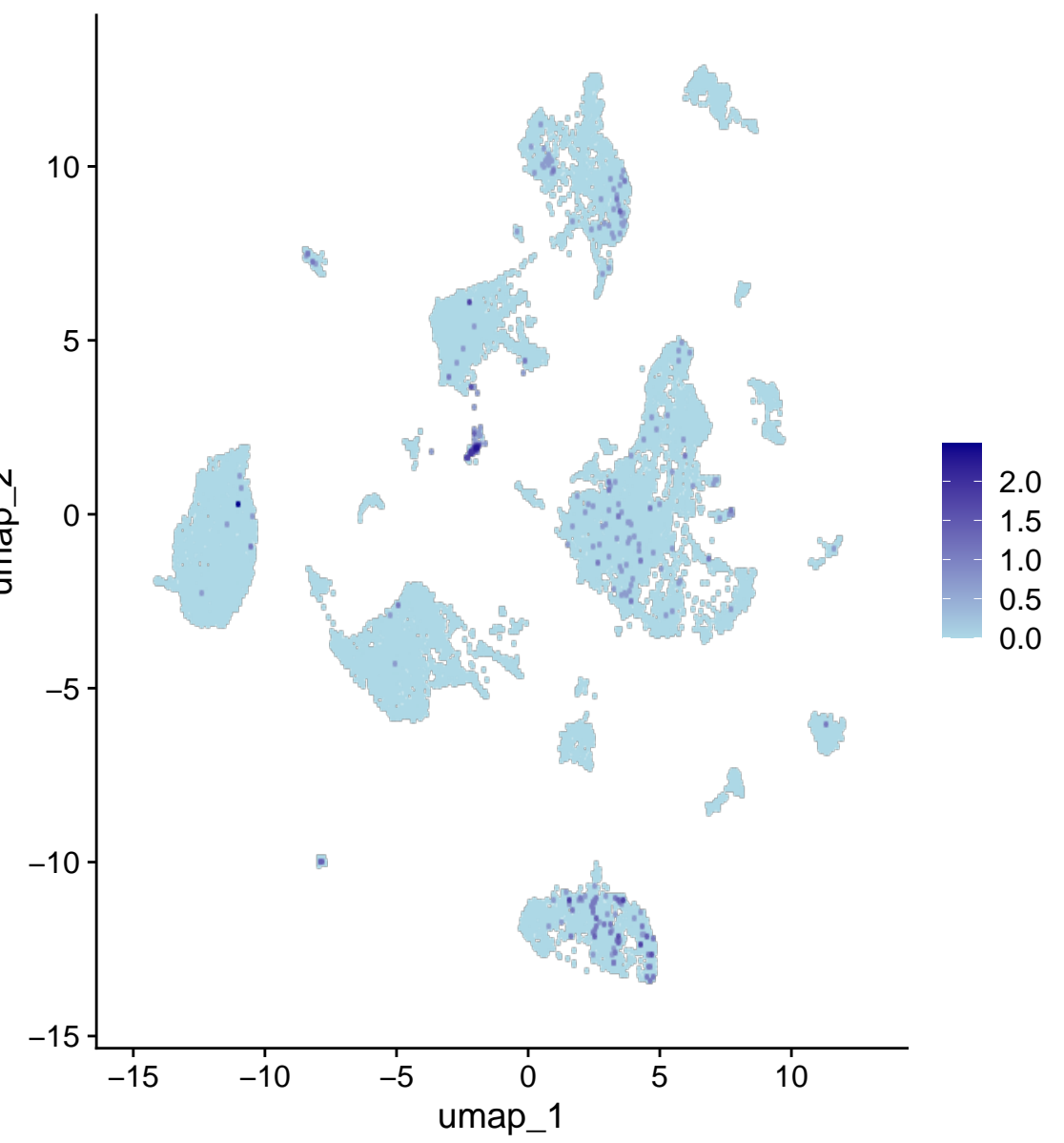
Slc7a11
