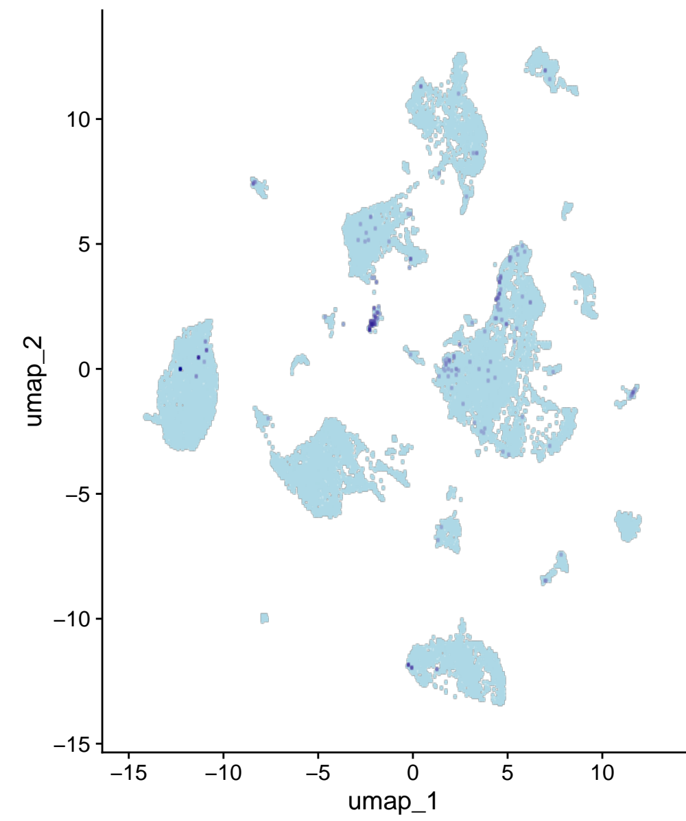
Gm6145
