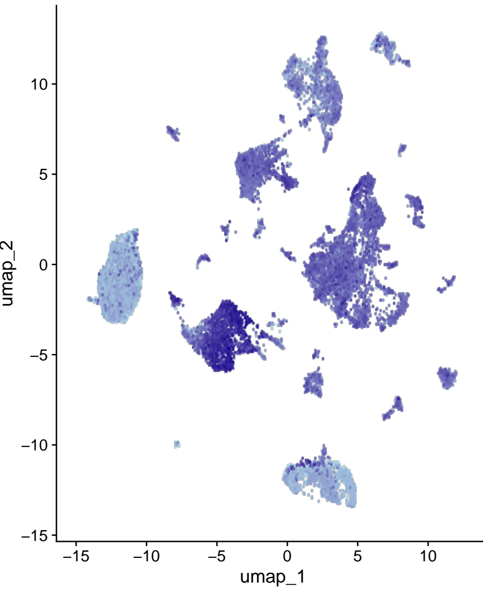
Pbx1
