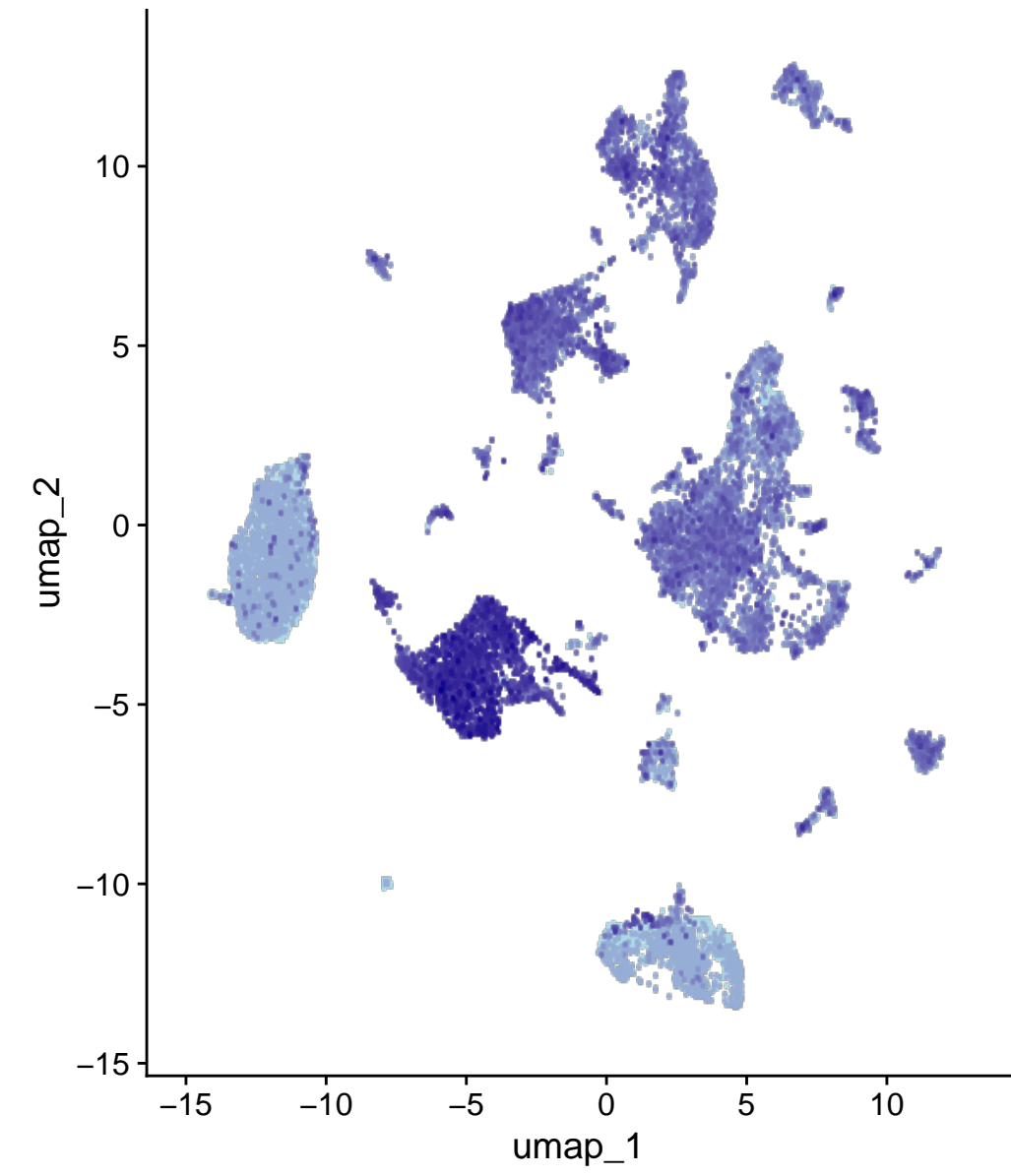
Cacna1c
