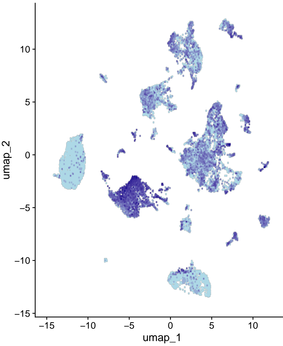
Prkg1
