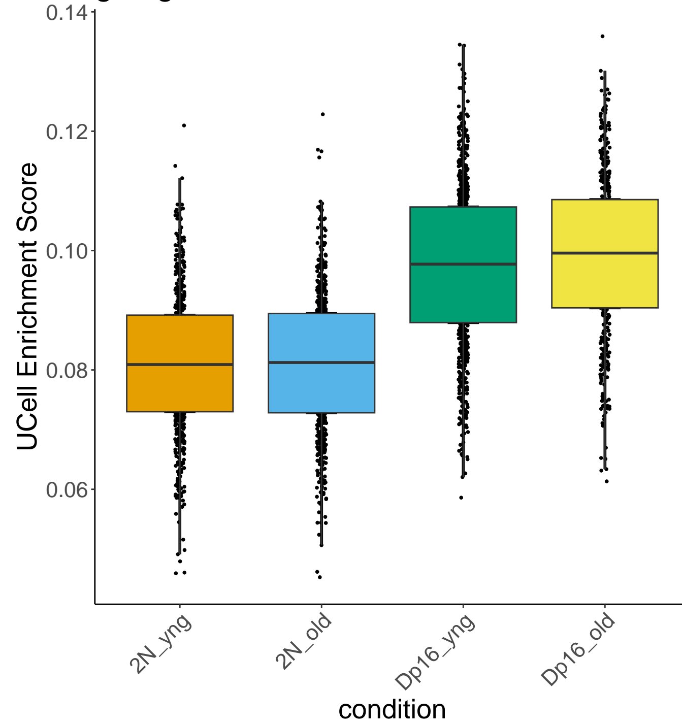
glut.gaba_2 : Tri16_UCell
