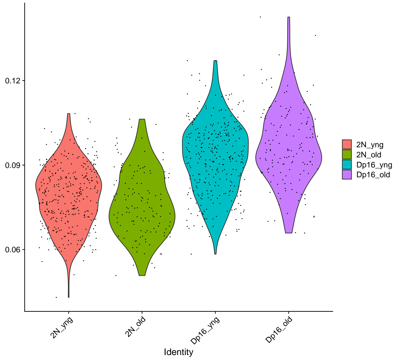
astrocyte2 : Tri16_UCell
