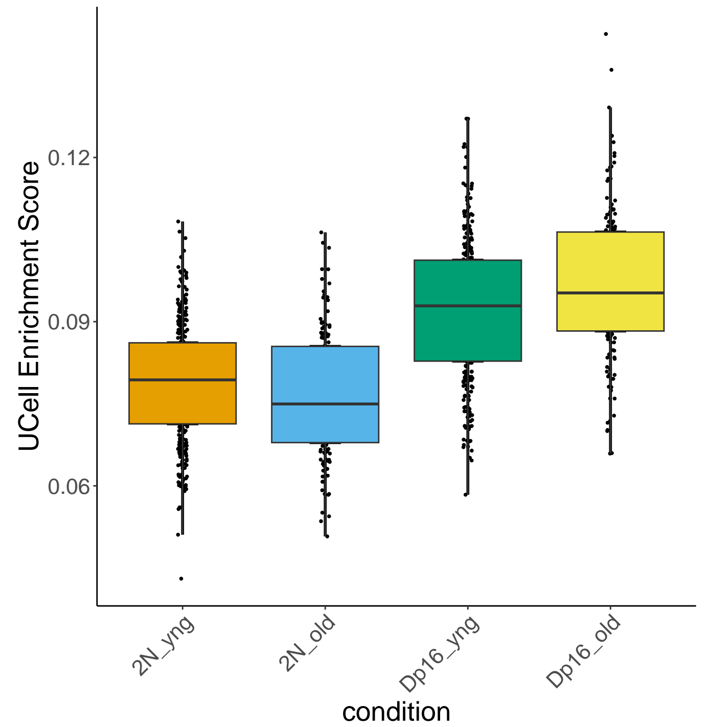
astrocyte2 : Tri16_UCell
