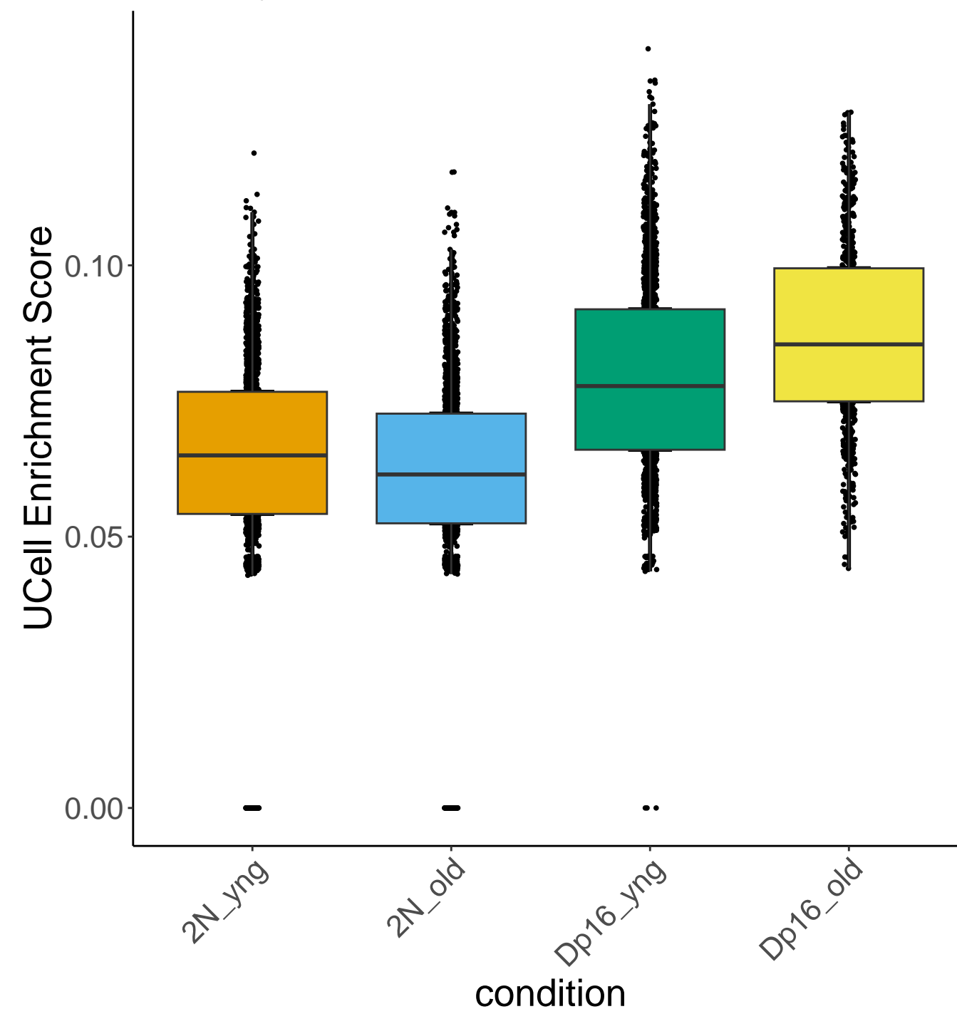
astrocyte1 : Tri16_UCell
