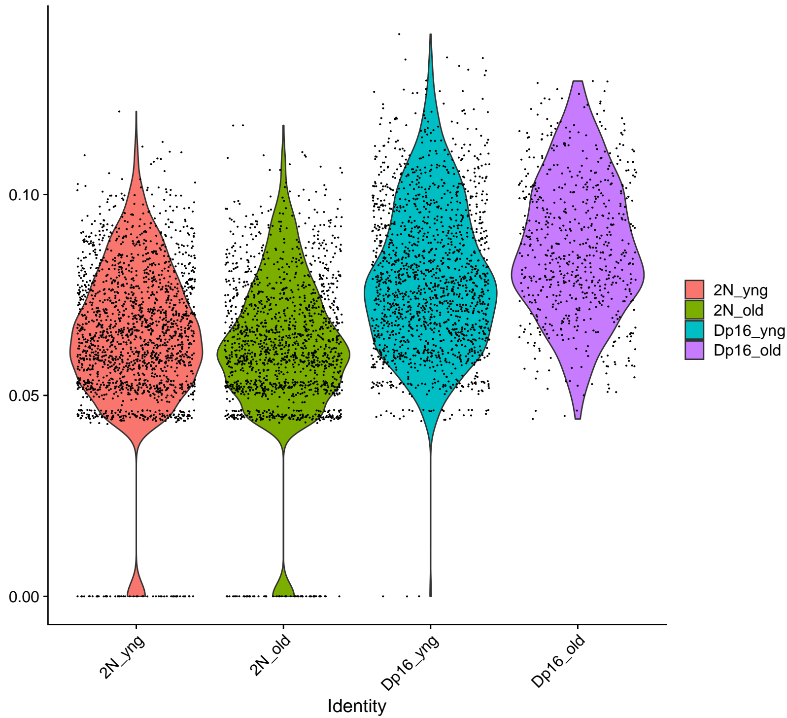
astrocyte1 : Tri16_UCell
