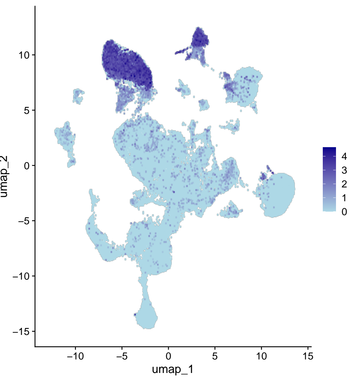
Sema3d
