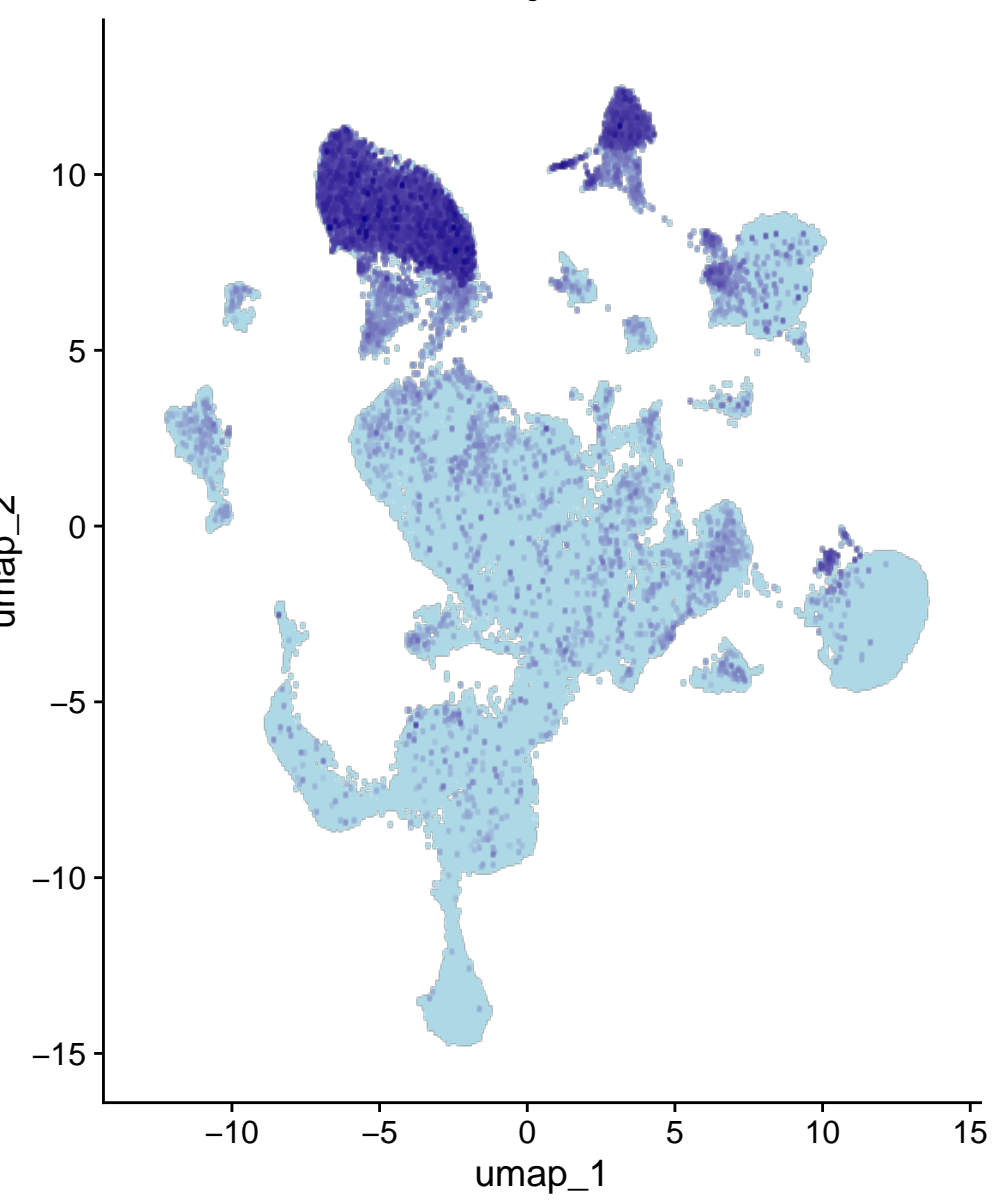
Kank1
