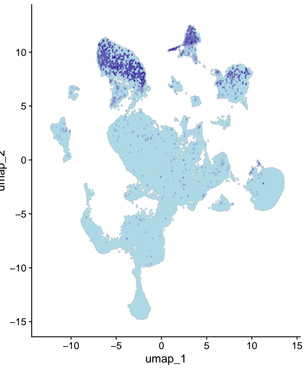
Bcas1os2
