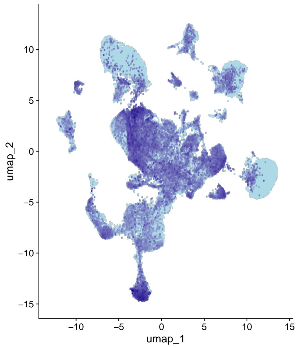
Grm8
