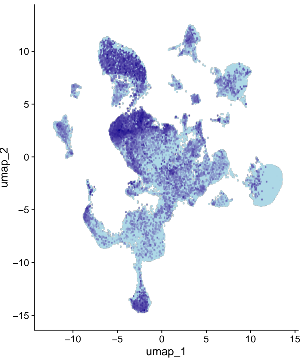
2010300C02Rik
