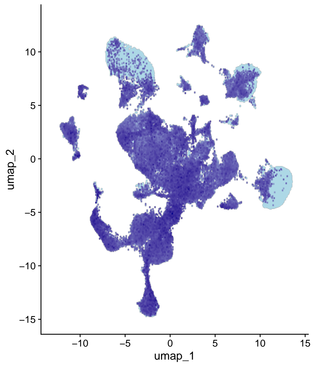
Pcdh7
