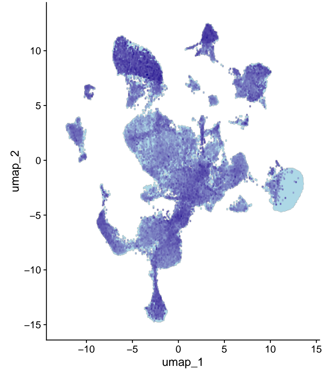
Prr16
