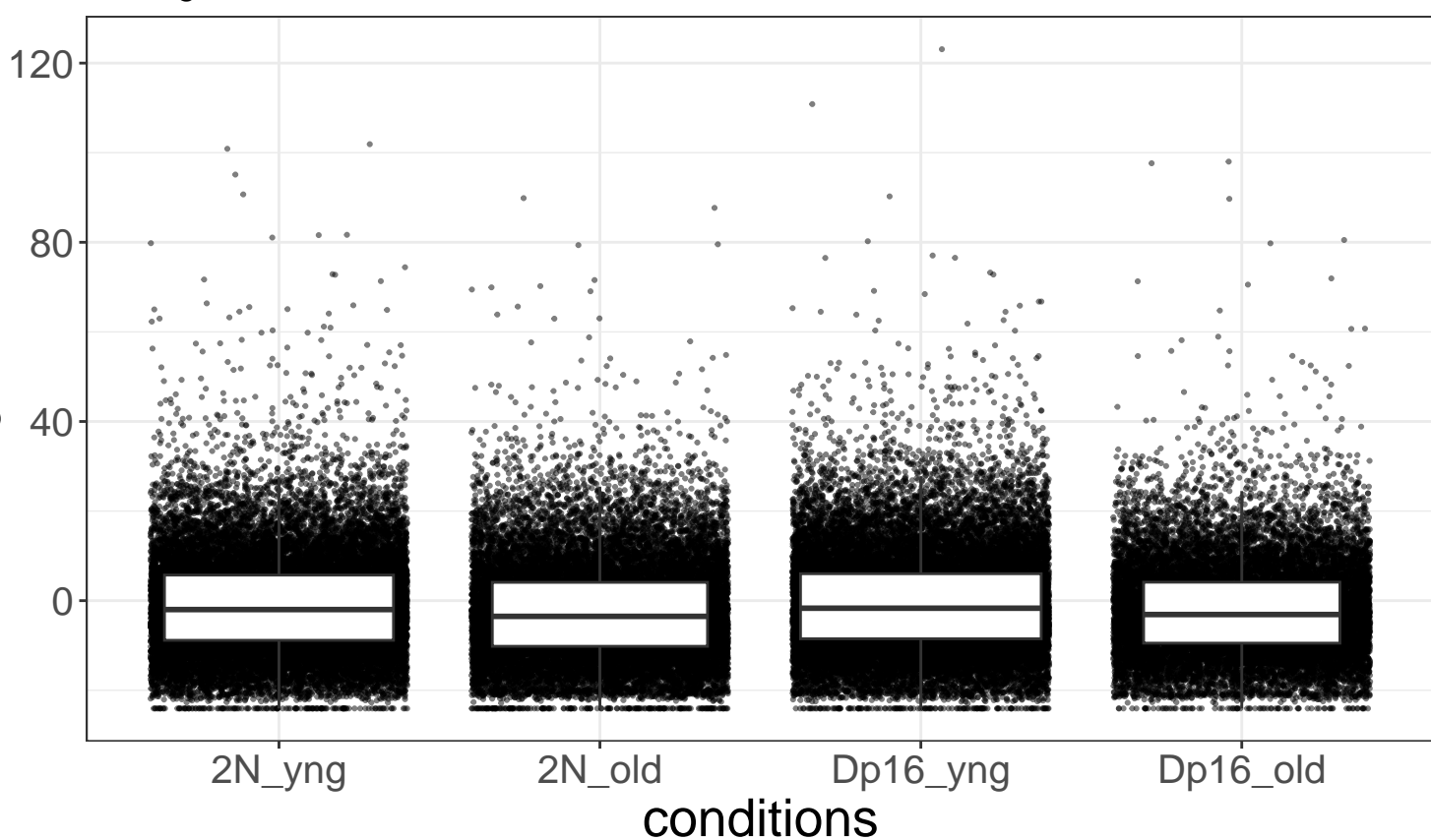
SenSig Scores: Global Scale
