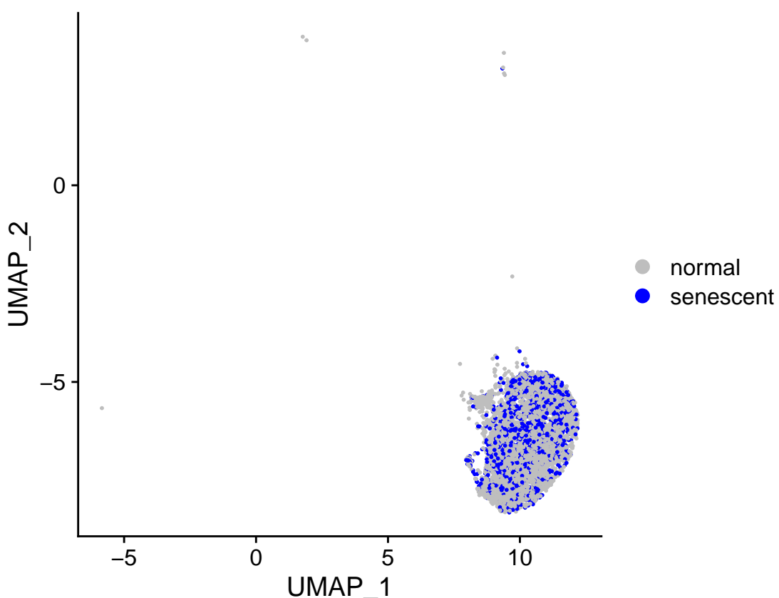
Cluster 7: sensig_150_bin_0.05_qsig
