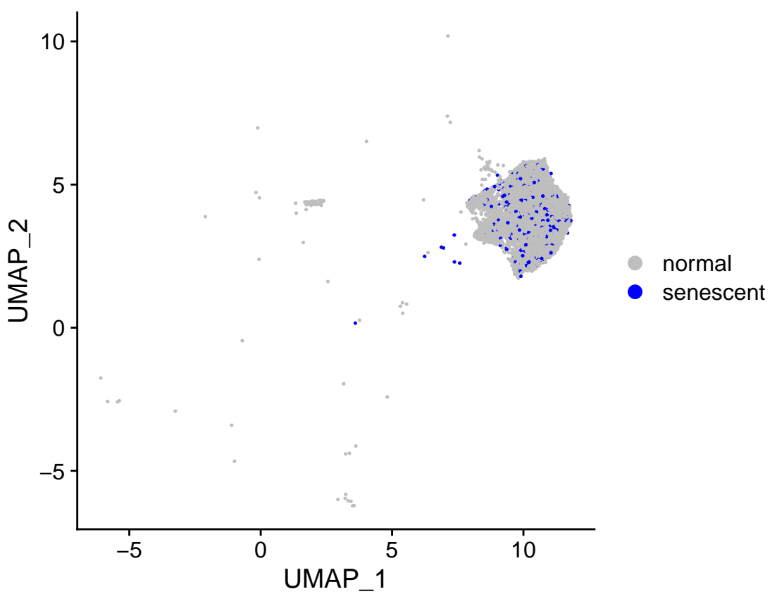
sensig_150_bin_0.05_qsig
