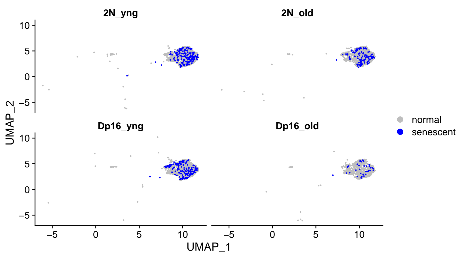
SenSig Scores
