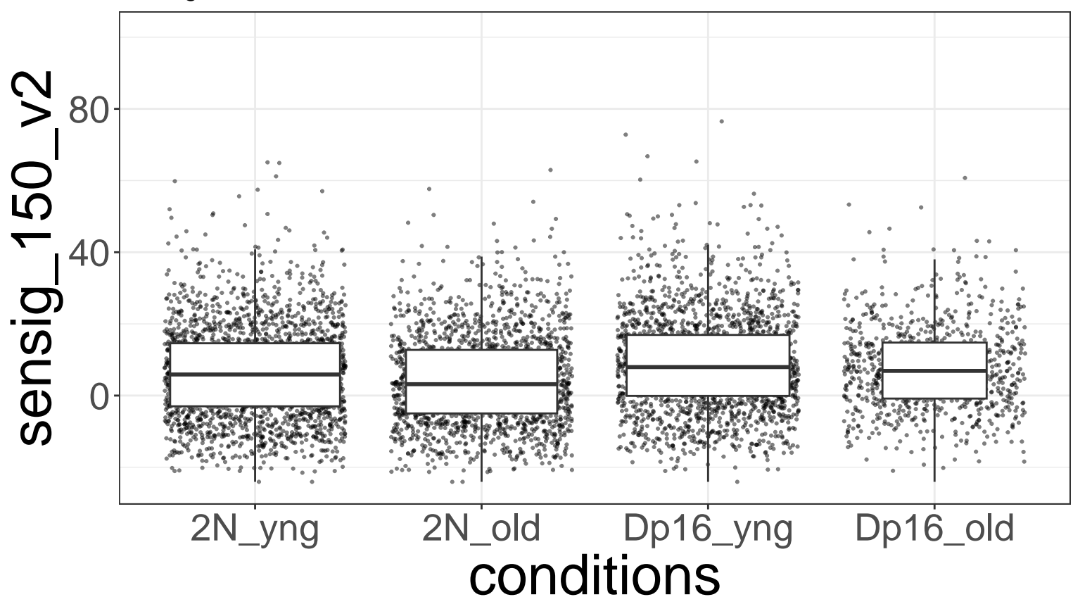
SenSig Scores
