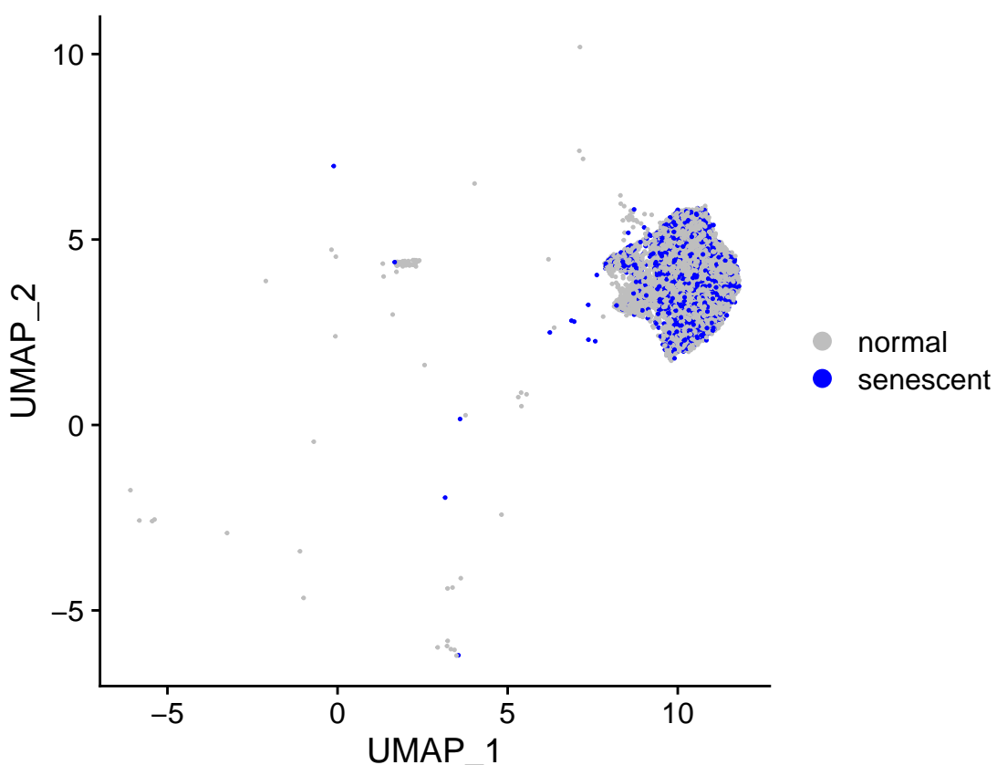
Cluster 4: sensig_150_bin_0.05_qsig
