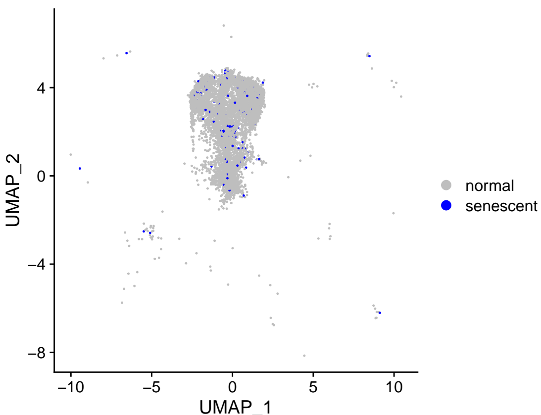
Cluster 3: sensig_150_bin_0.05_qsig
