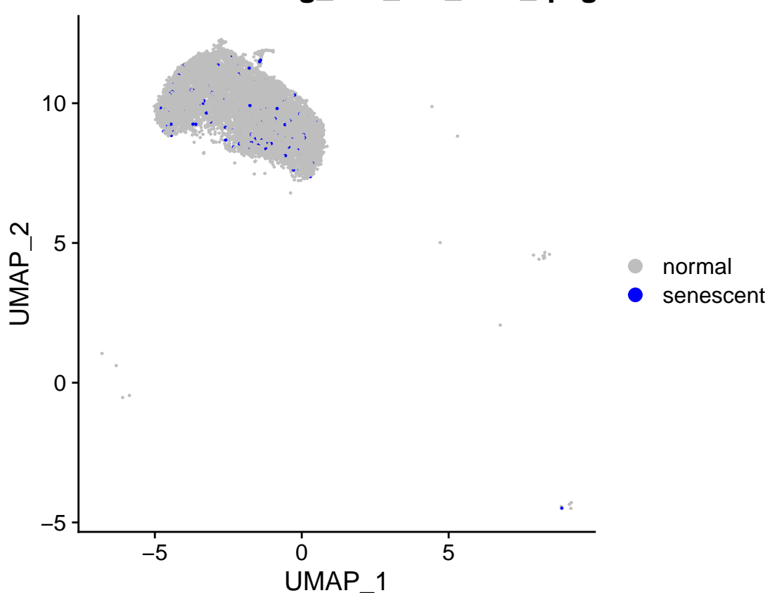
sensig_150_bin_0.05_qsig
