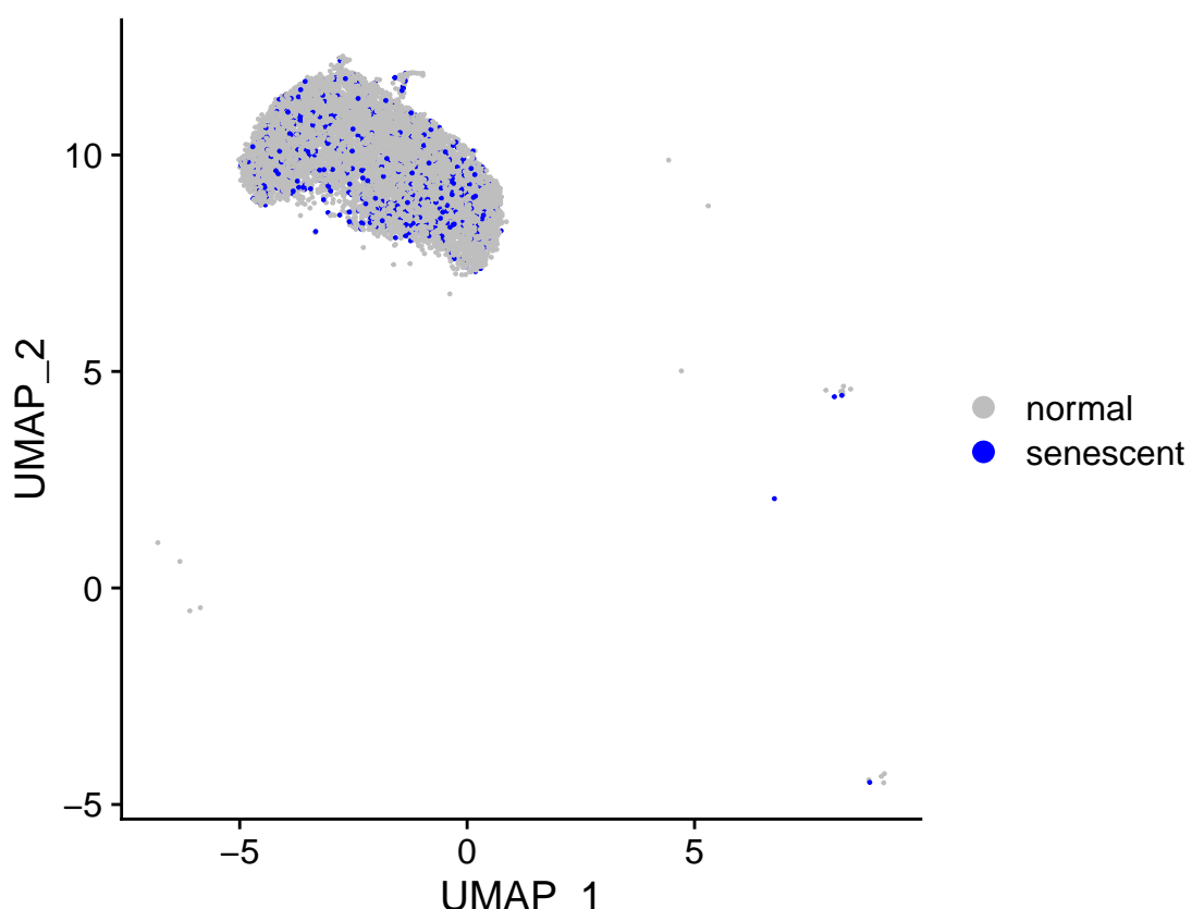
Cluster 2: sensig_150_bin_0.05_qsig
