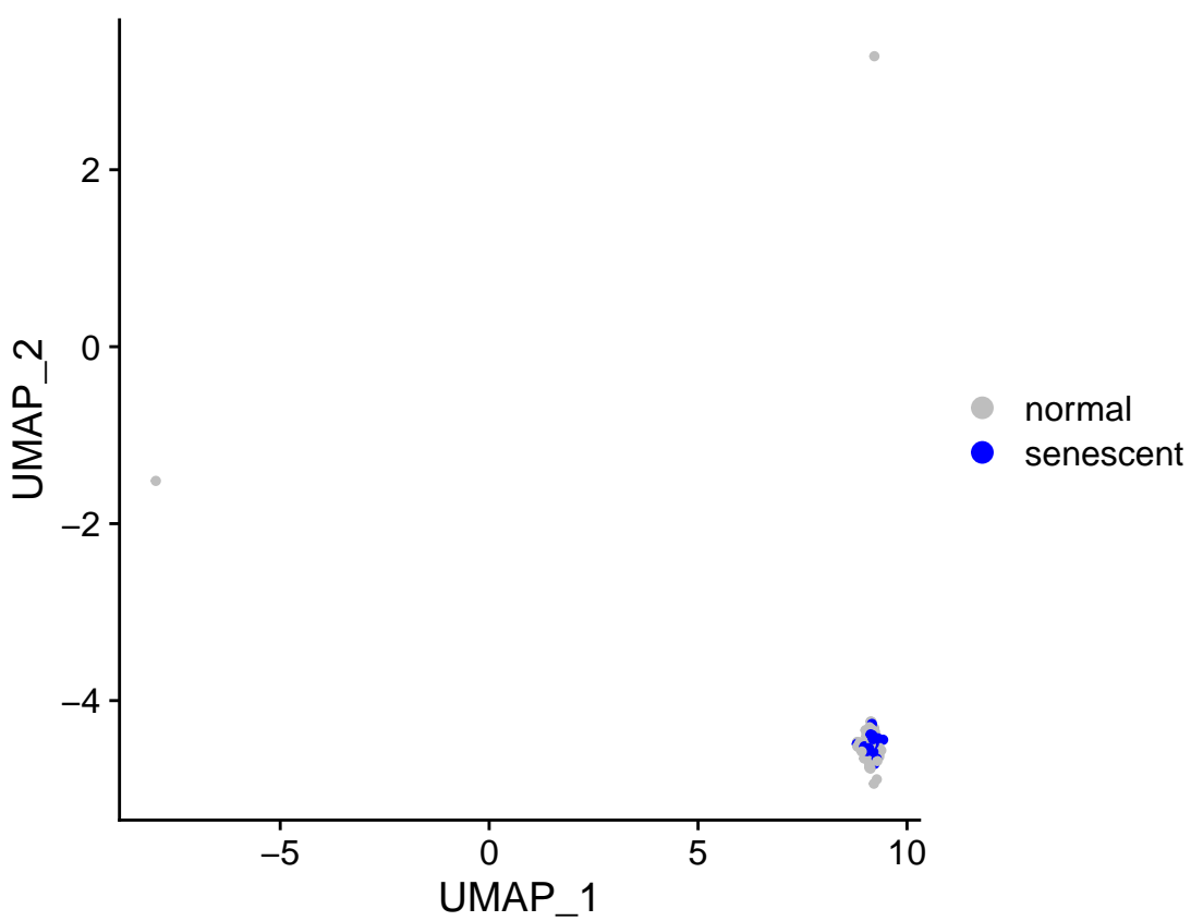
Cluster 24: sensig_150_bin_0.05_qsig
