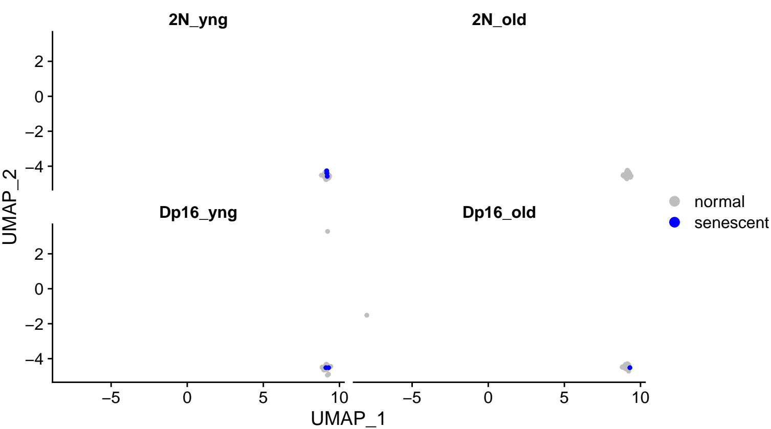
sensig_150_bin_0.05_qsig
