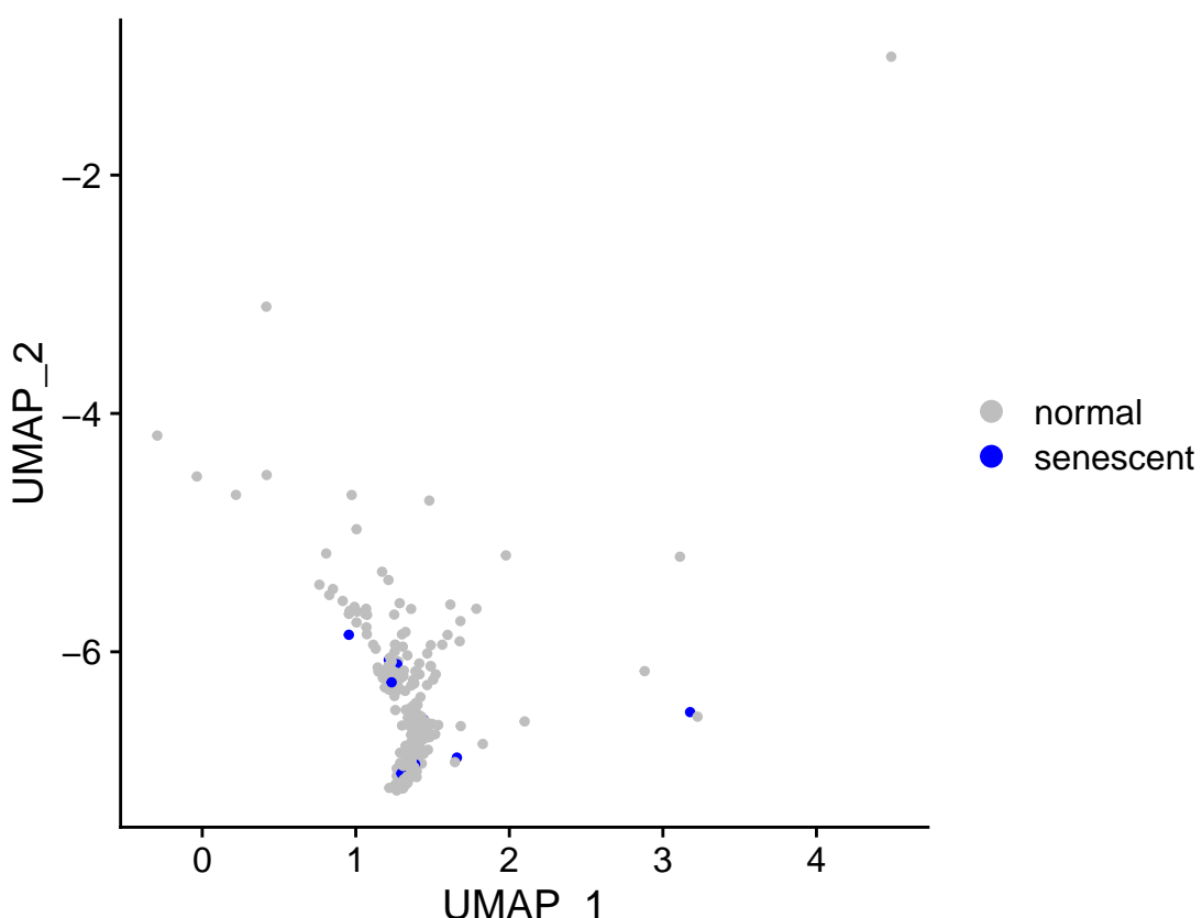
Cluster 23: sensig_150_bin_0.05_qsig
