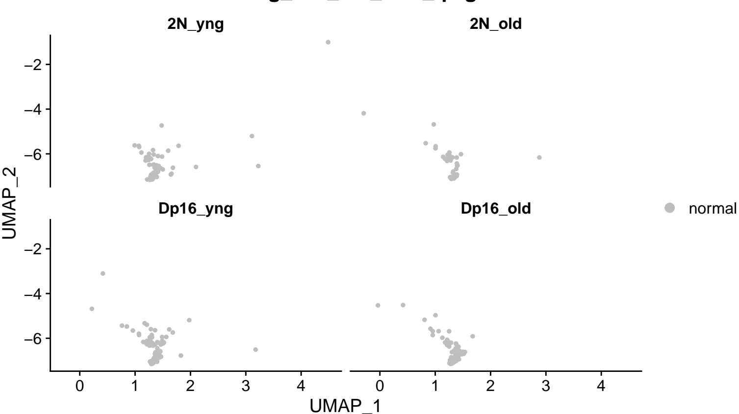
SenSig Scores
