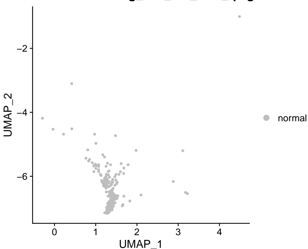
sensig_150_bin_0.05_qsig
