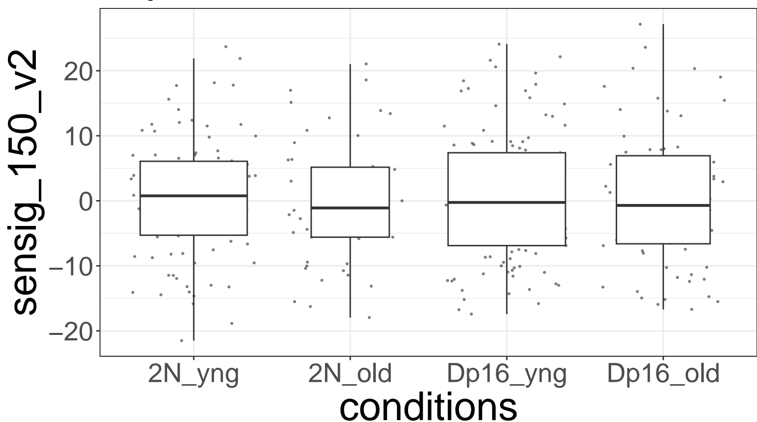
SenSig Scores
