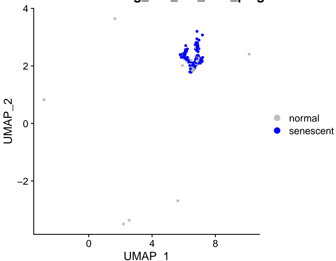
Cluster 22: sensig_150_bin_0.05_qsig
