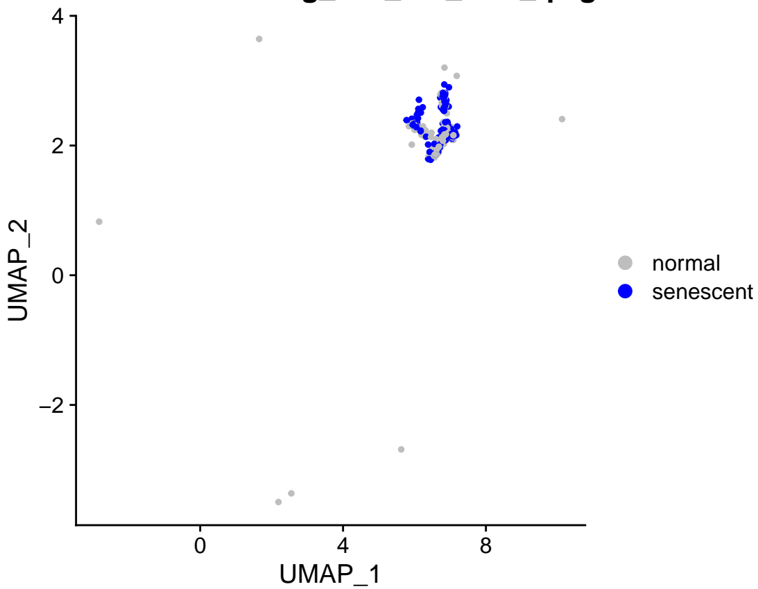
sensig_150_bin_0.05_qsig
