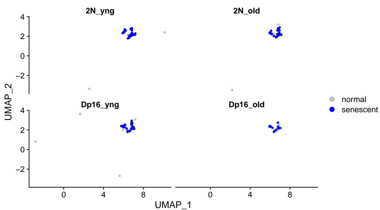
sensig_150_bin_0.05_qsig
