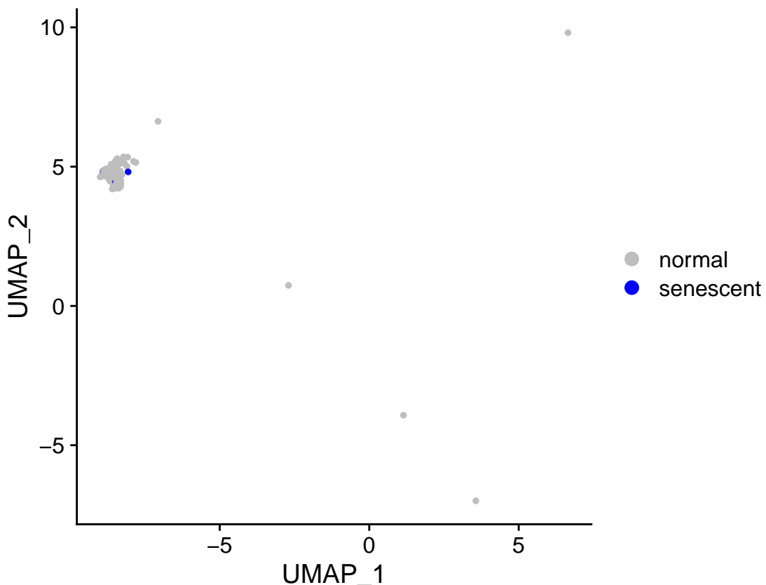
Cluster 21: sensig_150_bin_0.05_qsig
