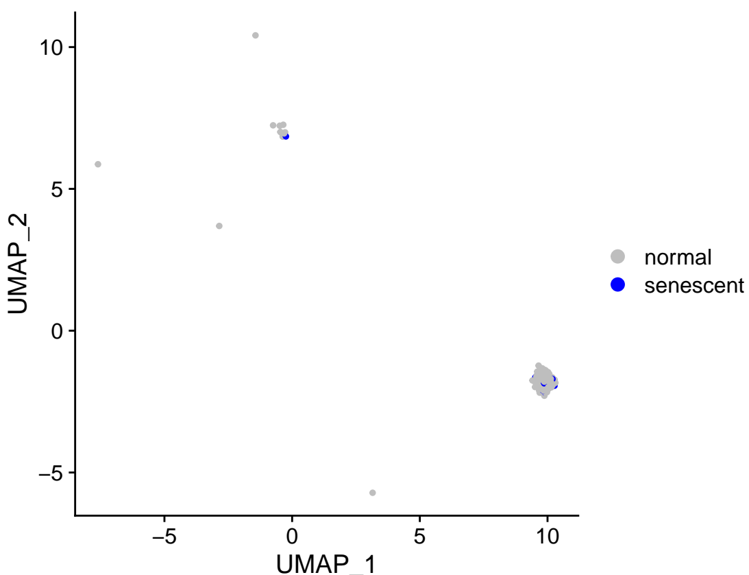
Cluster 19: sensig_150_bin_0.05_qsig
