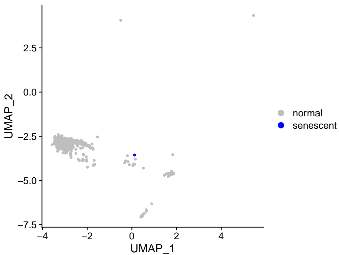
sensig_150_bin_0.05_qsig
