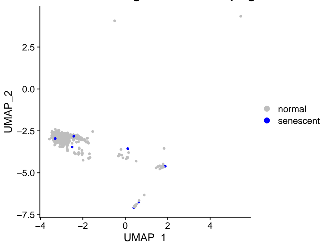
Cluster 18: sensig_150_bin_0.05_qsig
