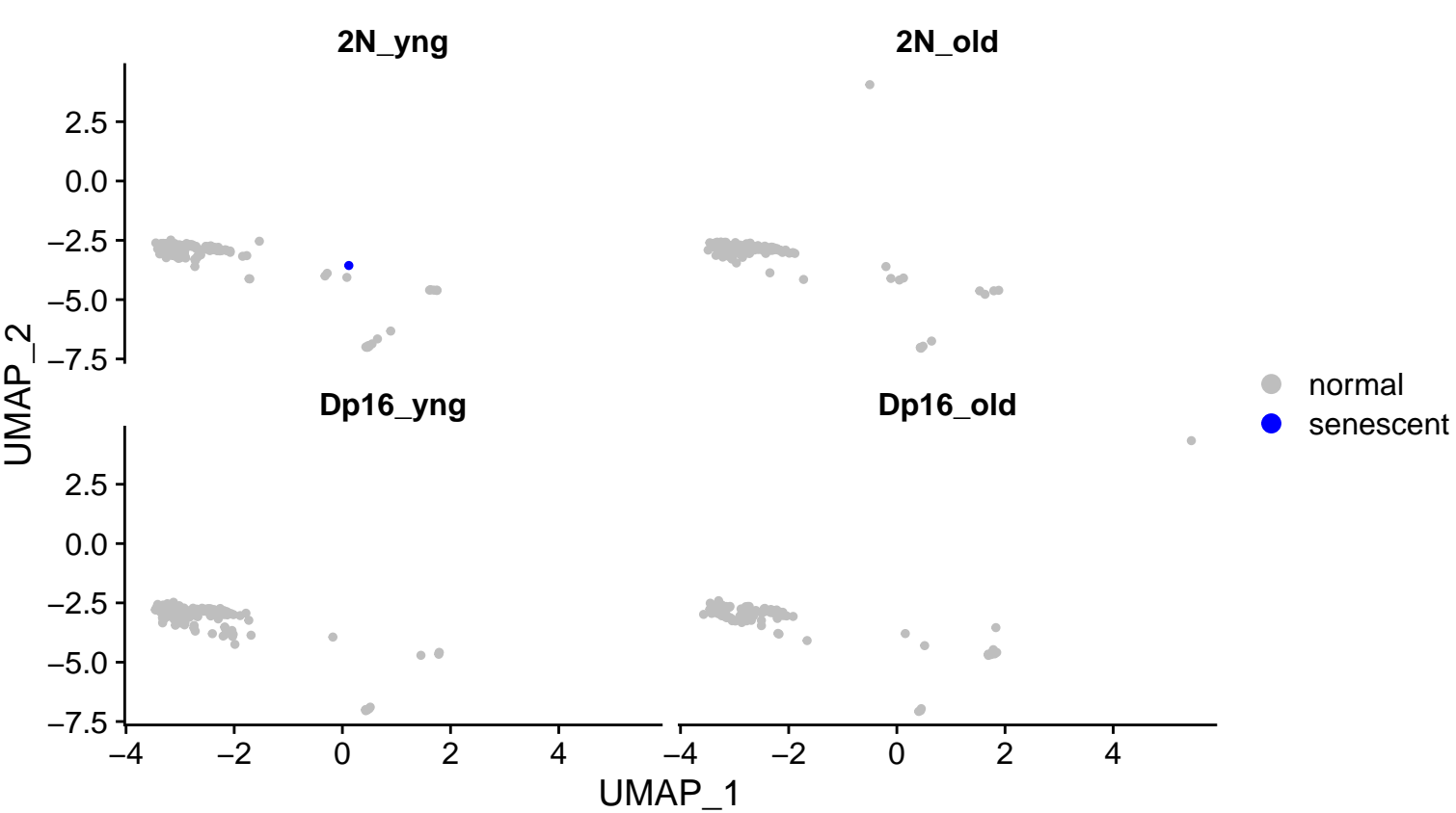
SenSig Scores
