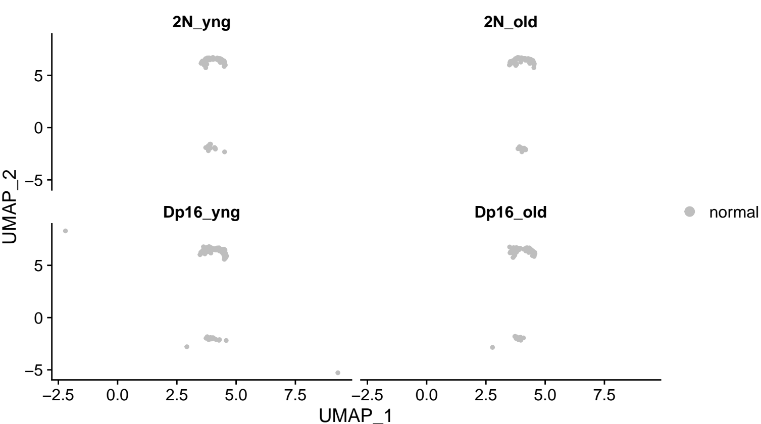
SenSig Scores
