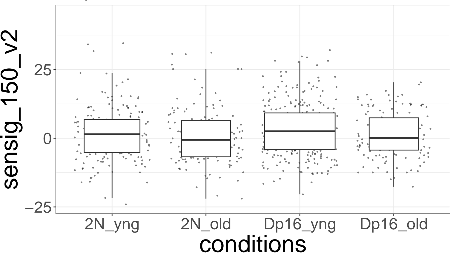
SenSig Scores
