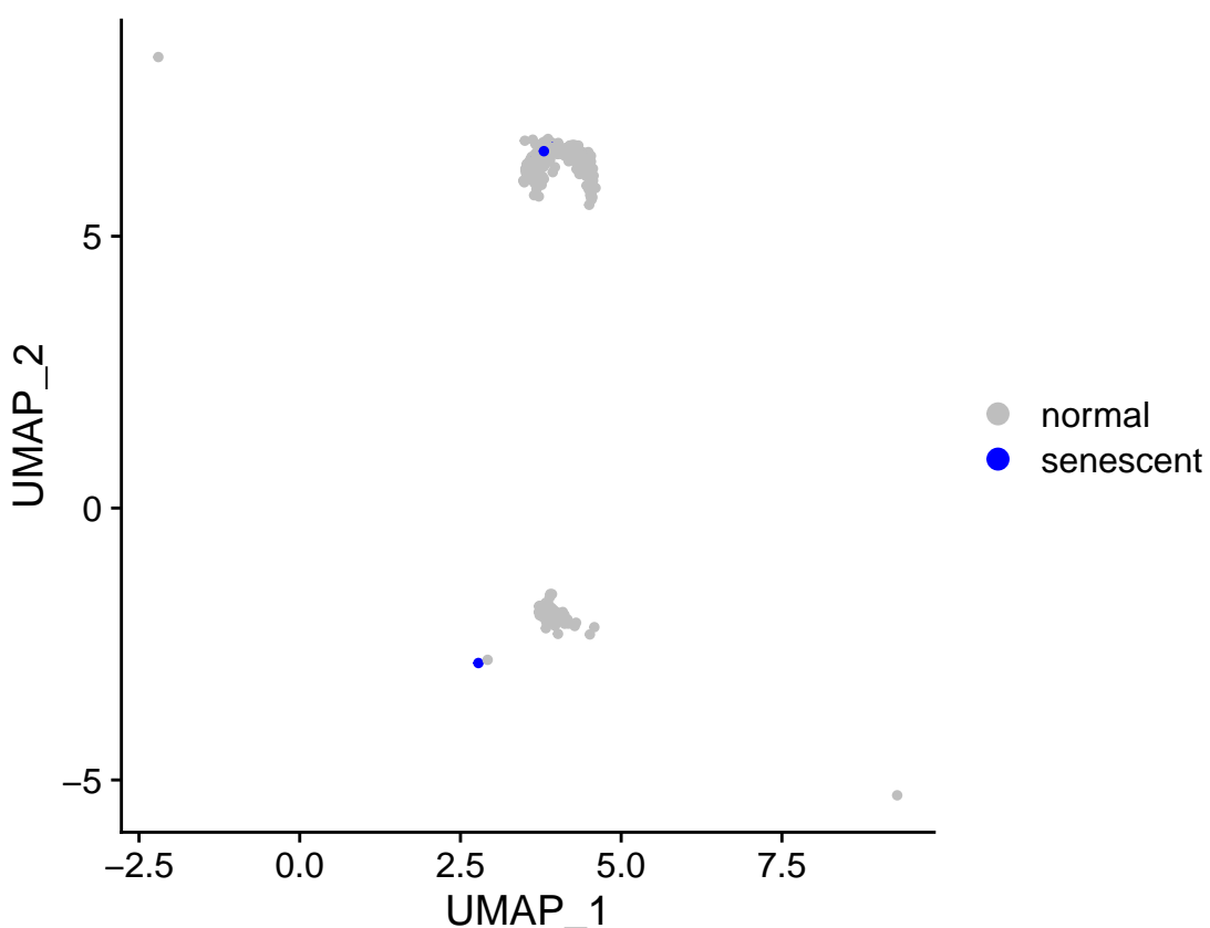
Cluster 17: sensig_150_bin_0.05_qsig
