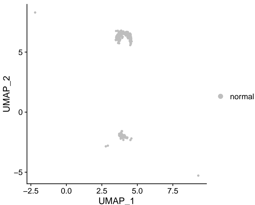
sensig_150_bin_0.05_qsig
