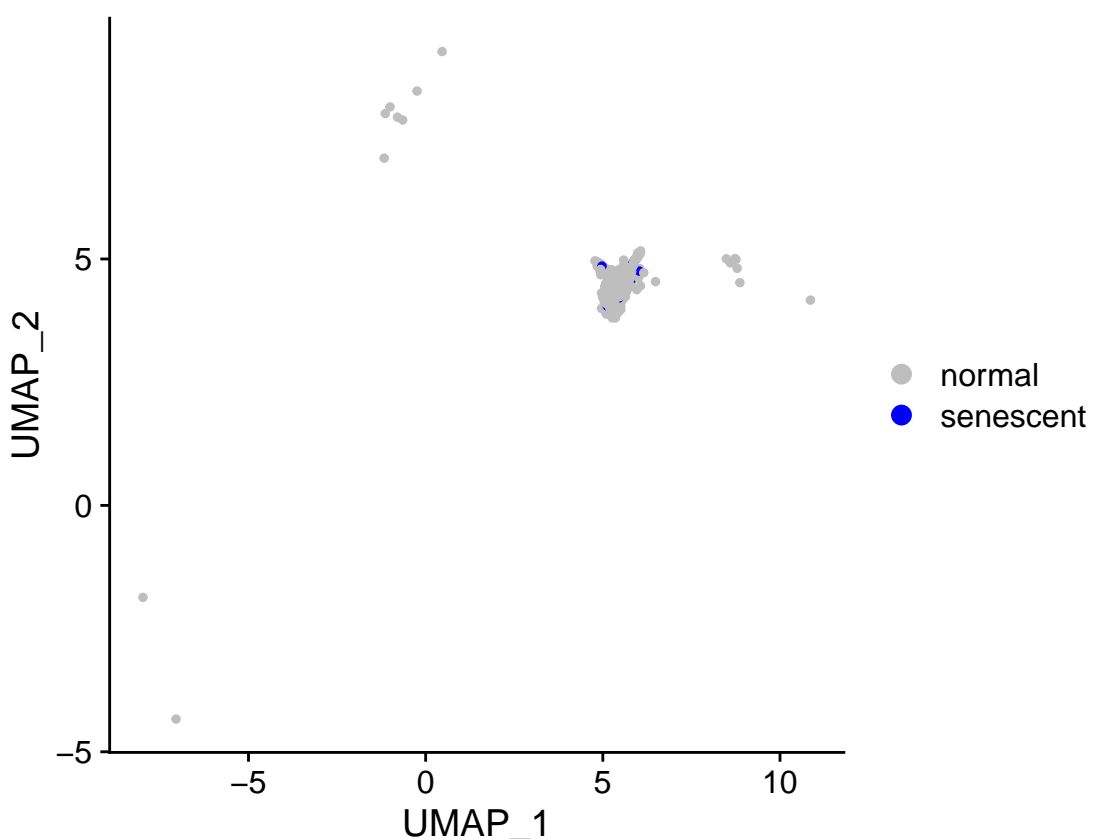
Cluster 16: sensig_150_bin_0.05_qsig
