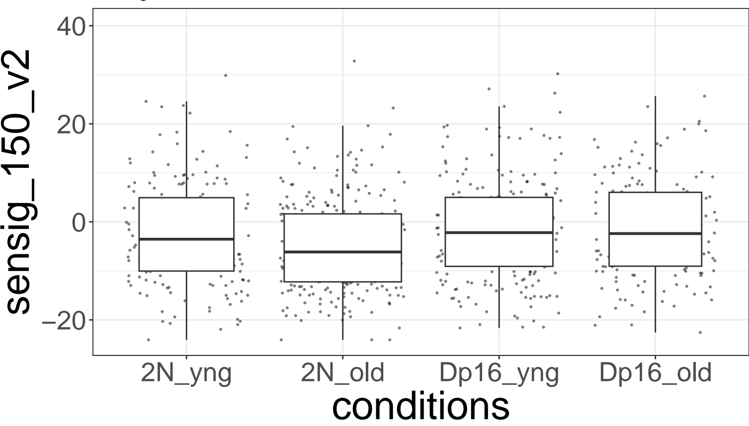
SenSig Scores
