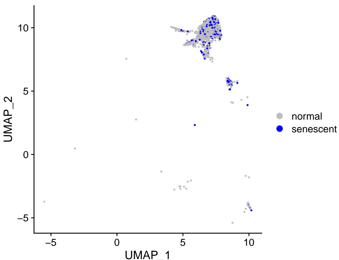
Cluster 10: sensig_150_bin_0.05_qsig
