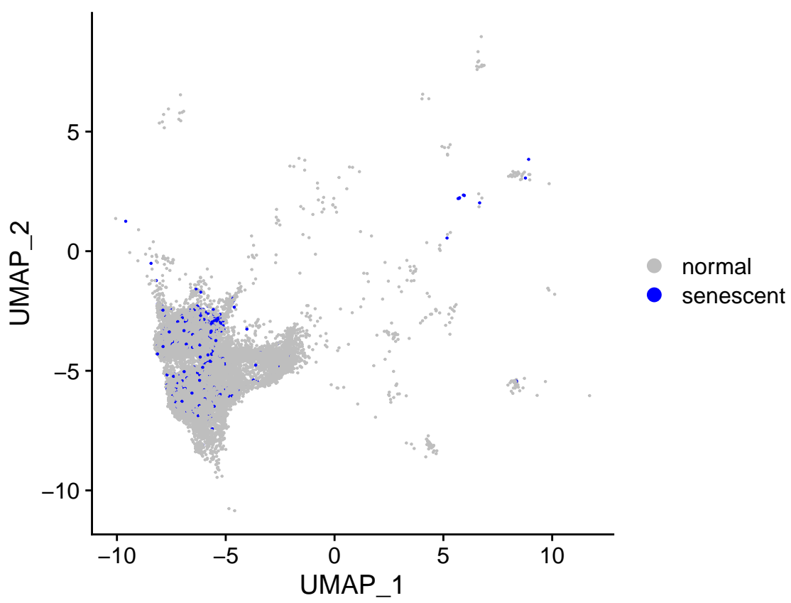
Cluster 0: sensig_150_bin_0.05_qsig
