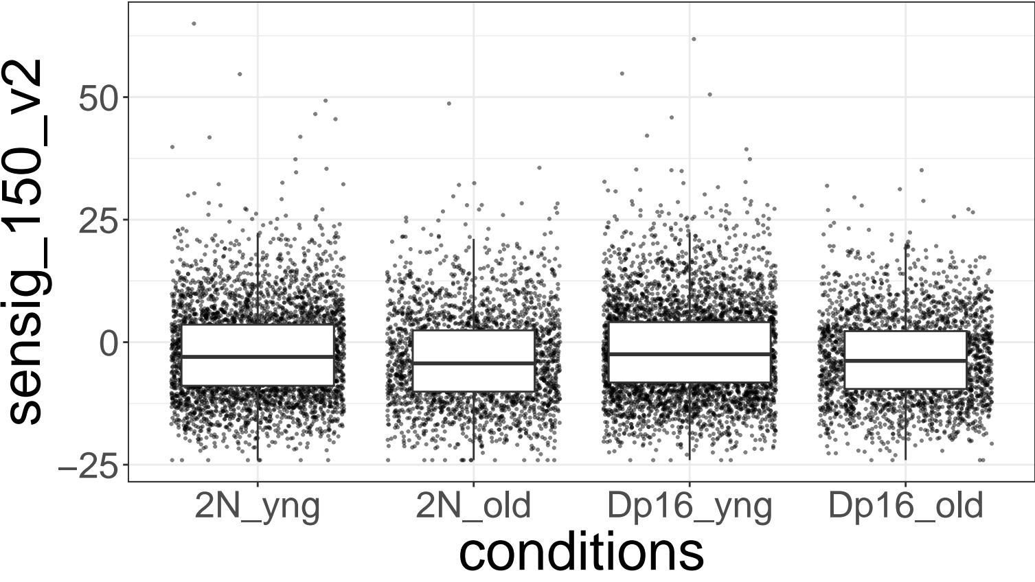
SenSig Scores
