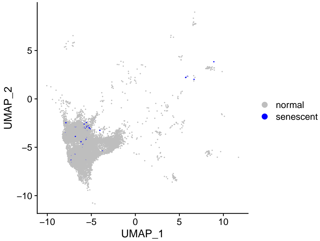
sensig_150_bin_0.05_qsig
