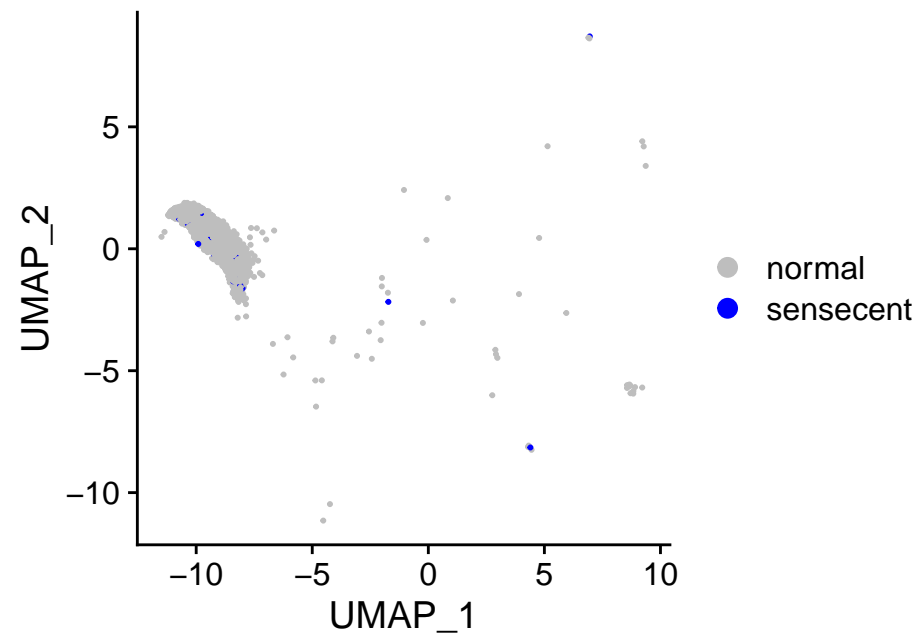
sensig_150_0.05_qsig
