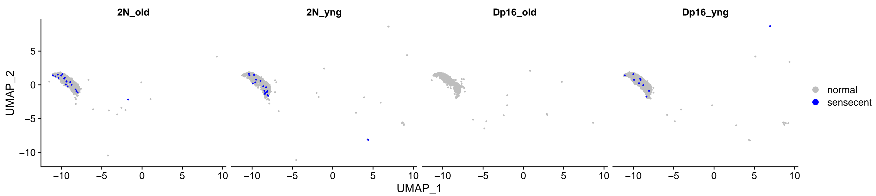
sensig_150_0.05_qsig
