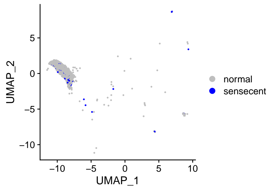
Cluster 9: sensig_150_0.05_qsig
