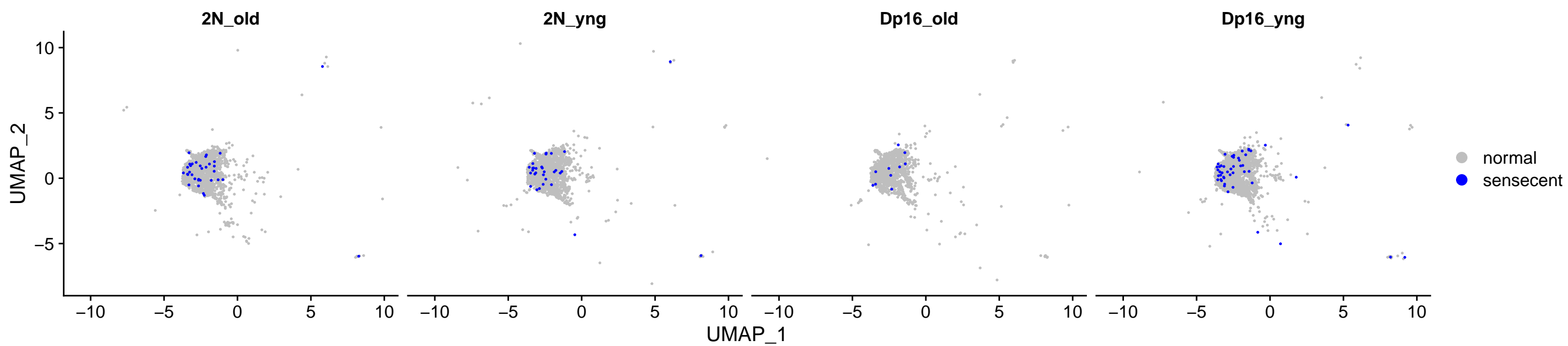
sensig_150_0.05_qsig
