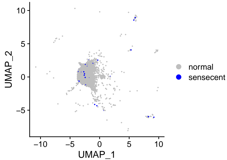
sensig_150_0.05_qsig
