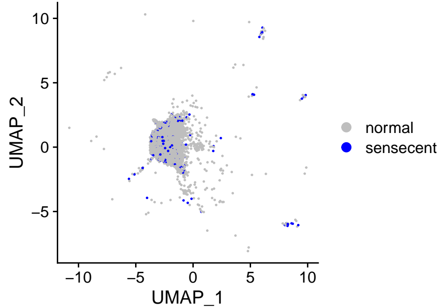
Cluster 5: sensig_150_0.05_qsig
