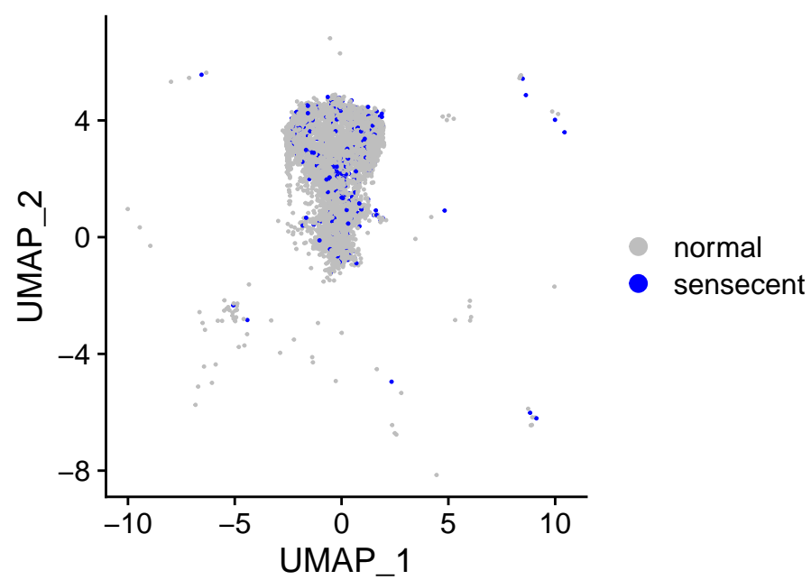
Cluster 3: sensig_150_0.05_qsig
