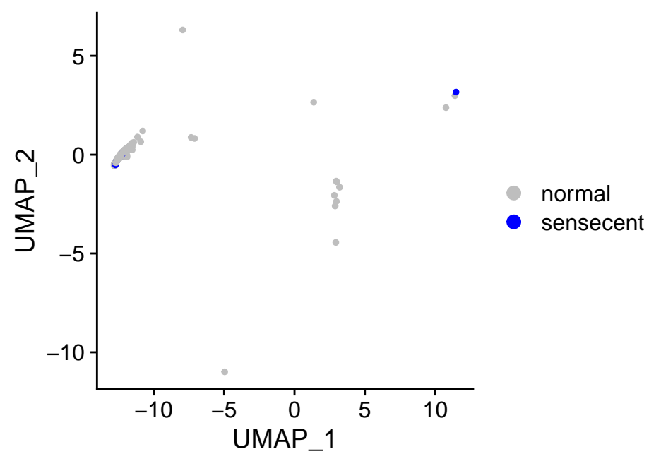
Cluster 20: sensig_150_0.05_qsig
