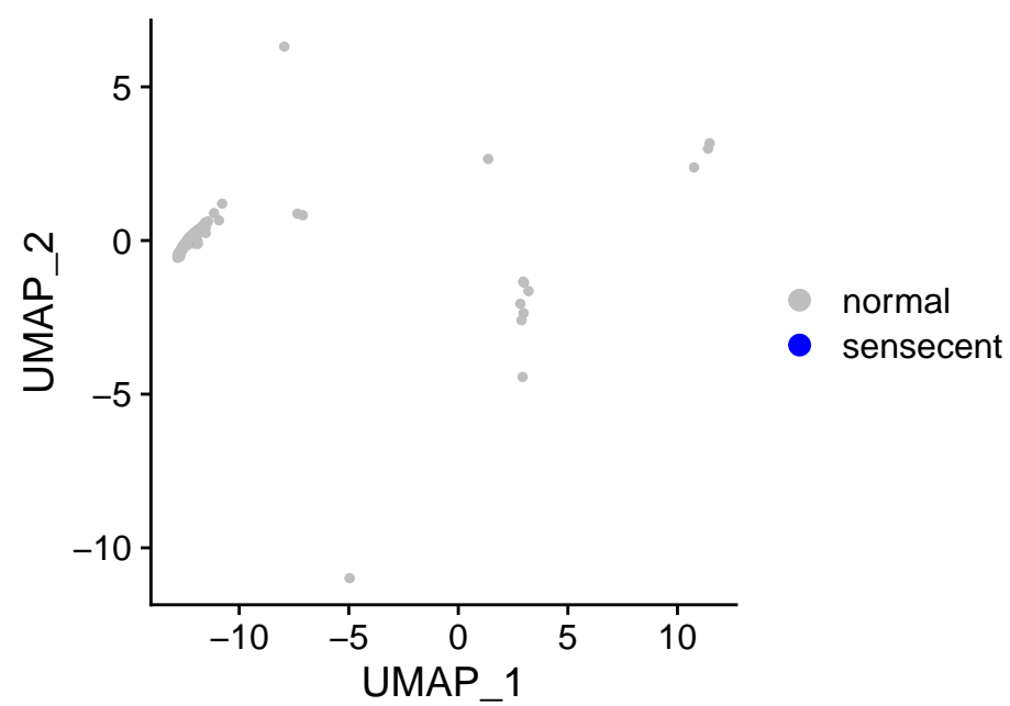
sensig_150_0.05_qsig
