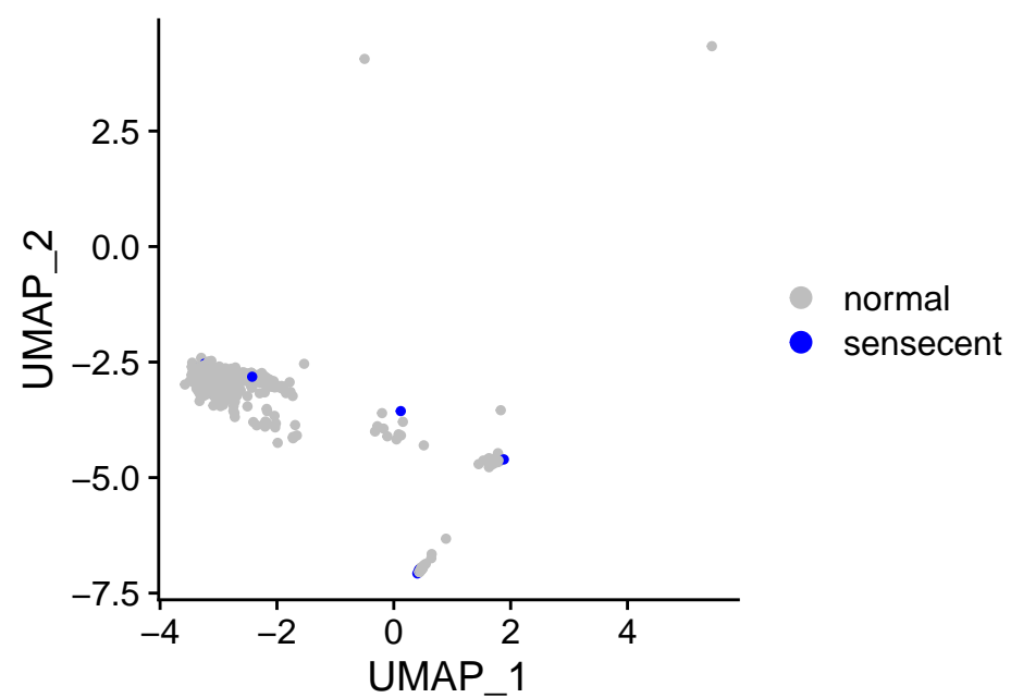
sensig_150_0.05_qsig
