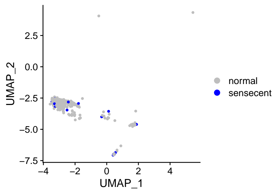
Cluster 18: sensig_150_0.05_qsig
