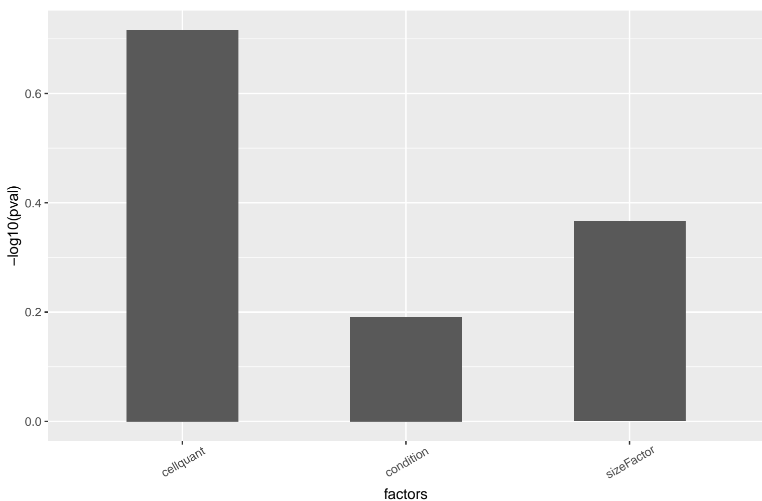
PC 2 vs covariates
