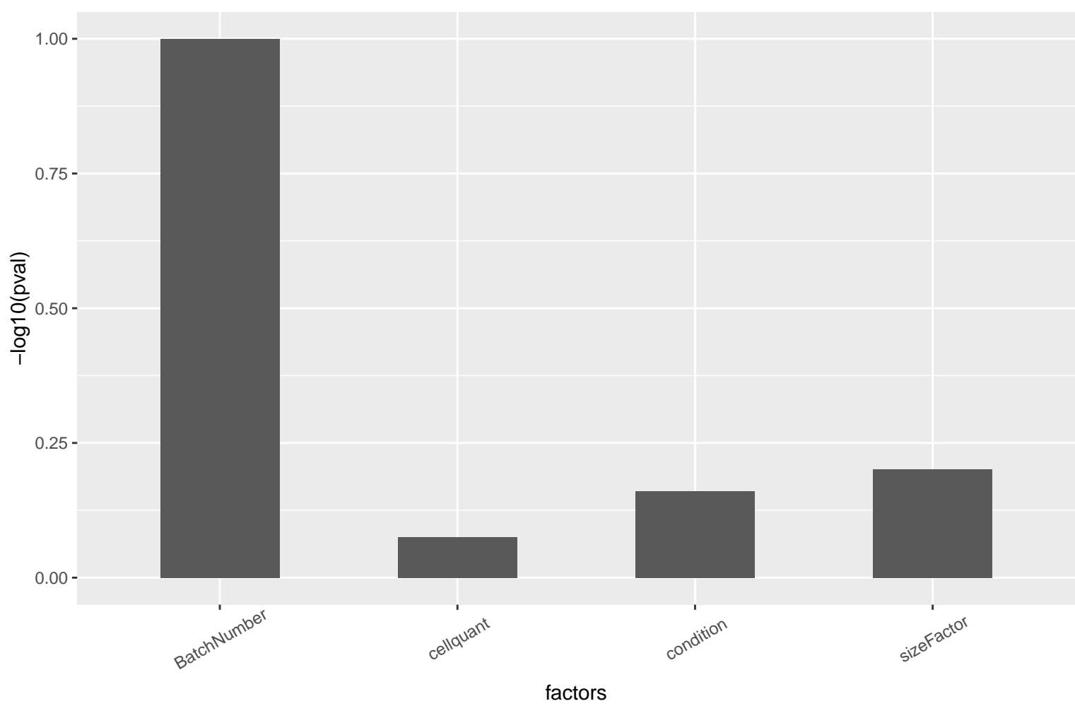
PC 2 vs covariates
