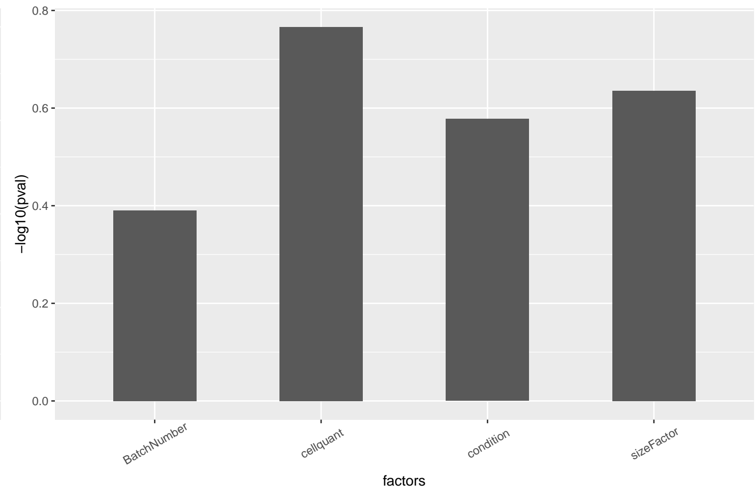
PC 4 vs covariates
