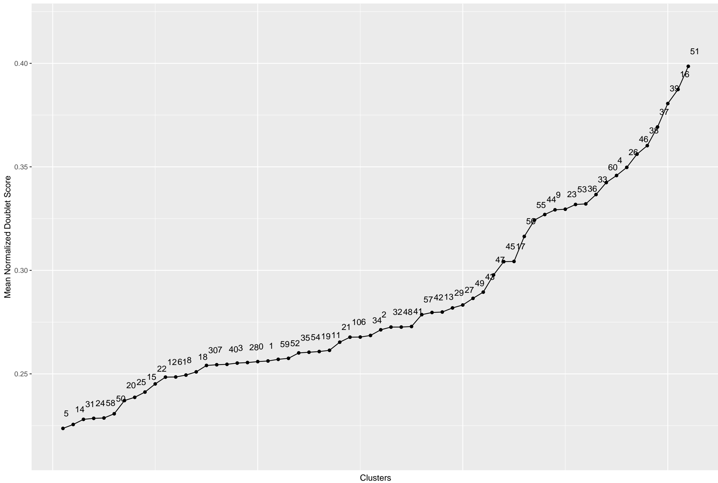
Mean Normalized Doublet Score per Cluster
