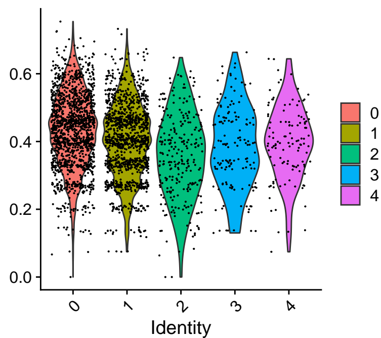
HM_v1_UCell
