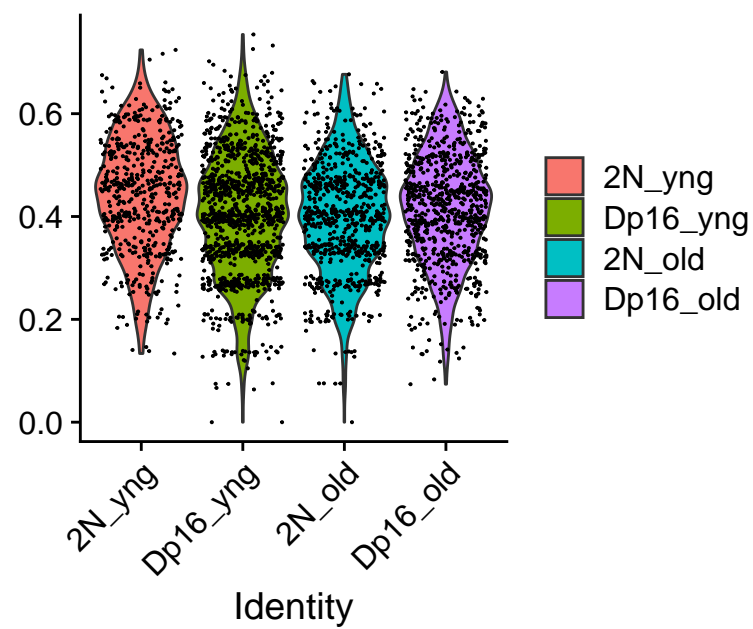
HM_v1_UCell
