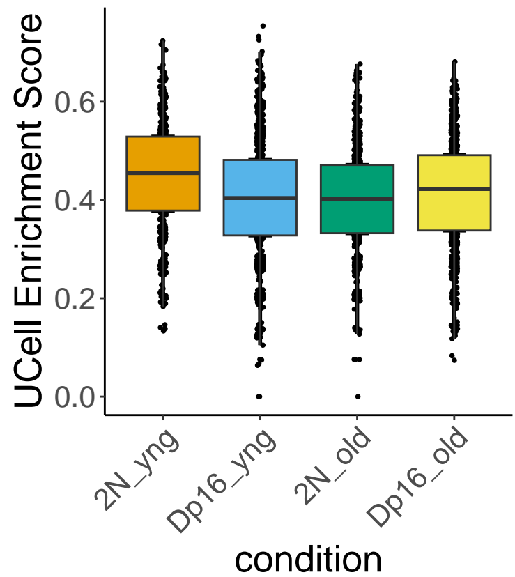
HM_v1_UCell
