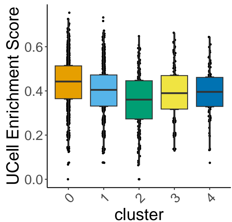
HM_v1_UCell
