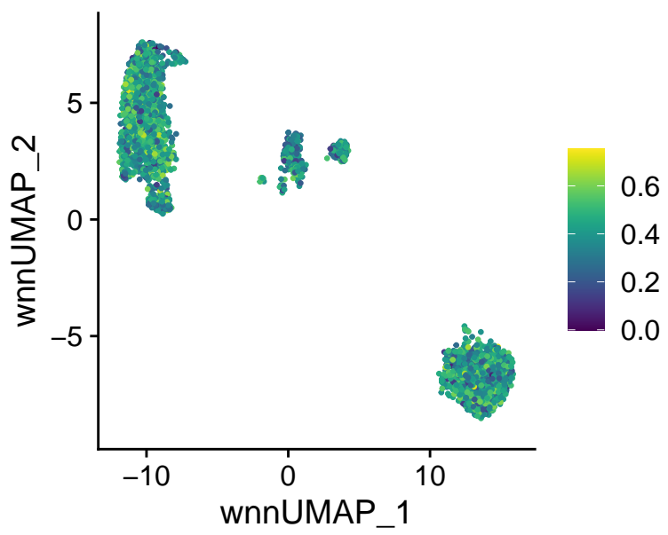
HM_v1_UCell
