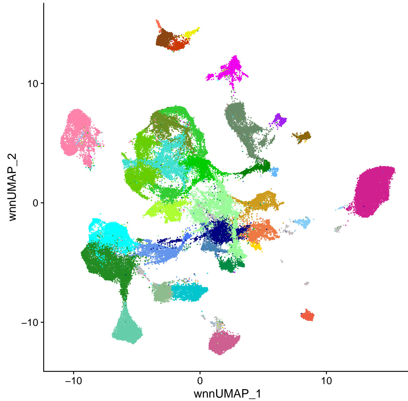
WNN
