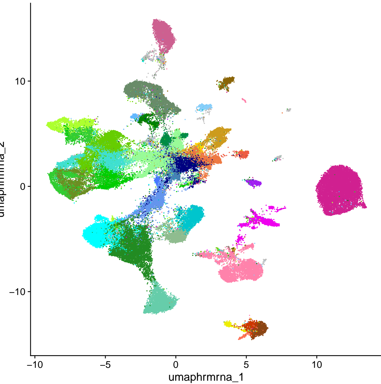
snRNA
