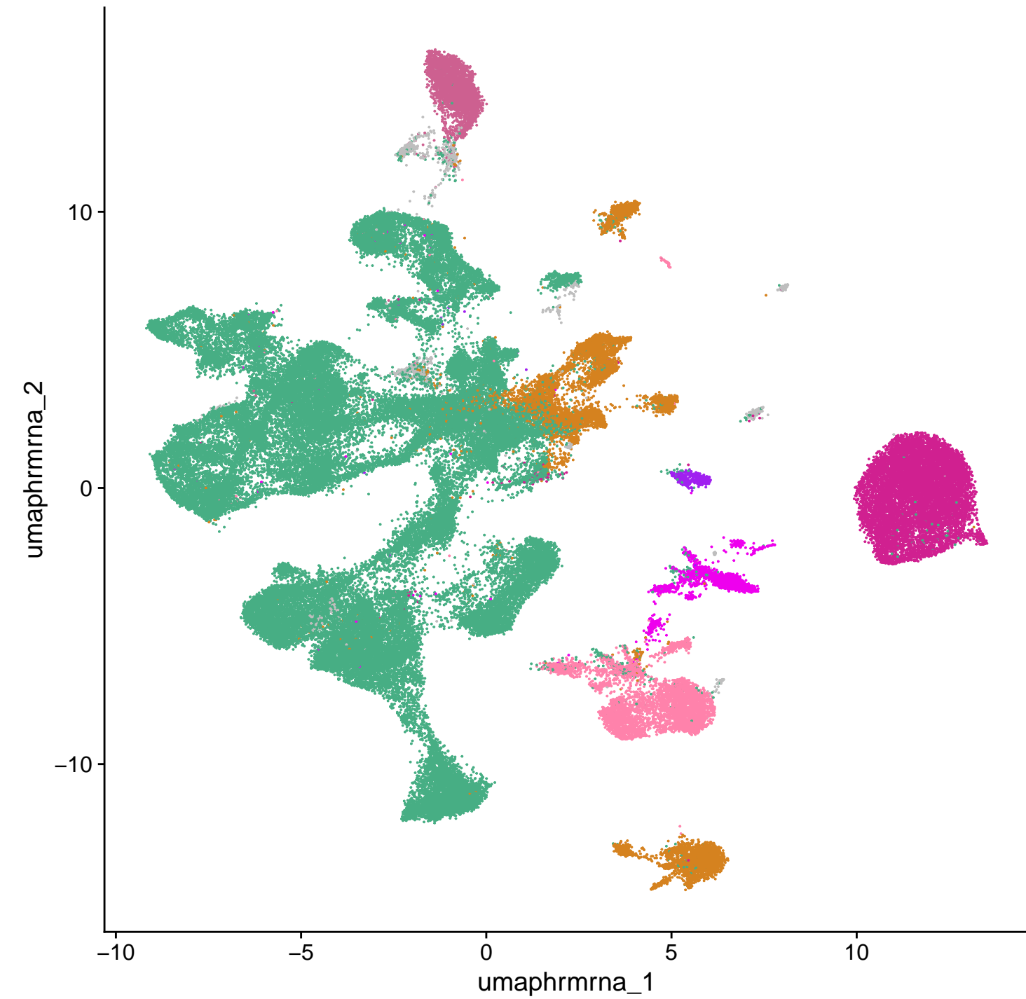
snRNA
