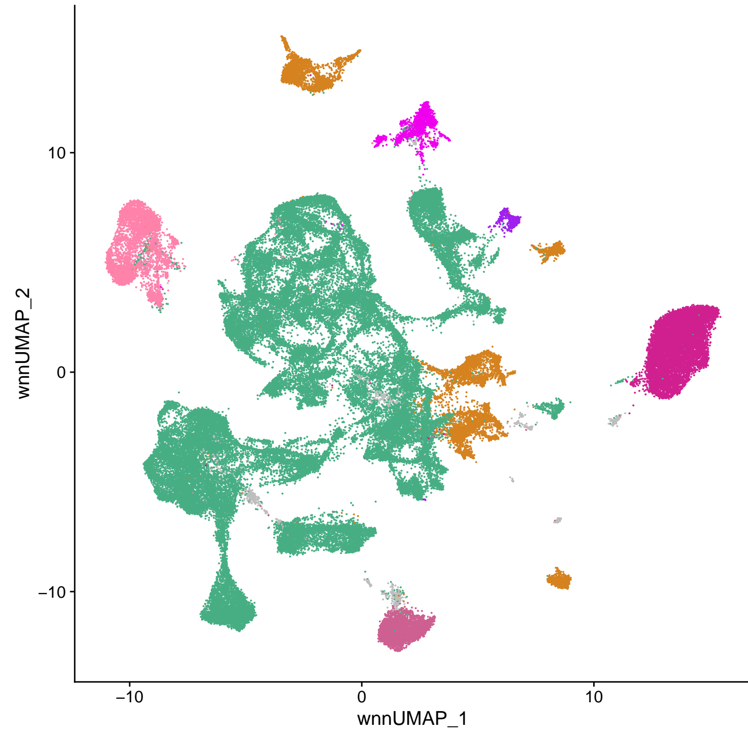
WNN
