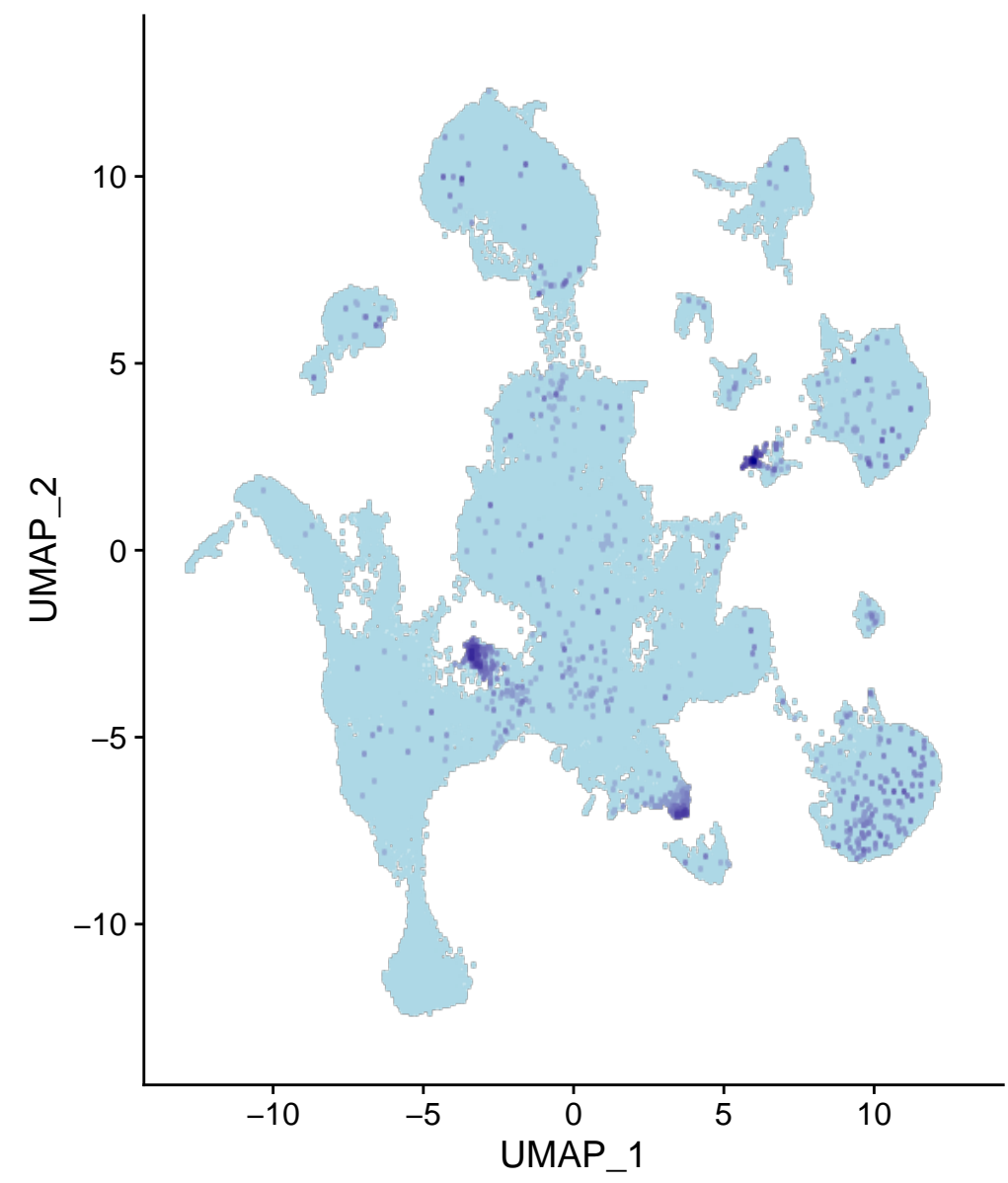
Dcc
