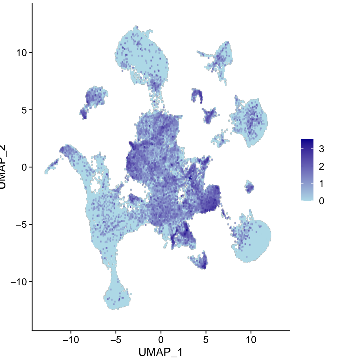
Acly
