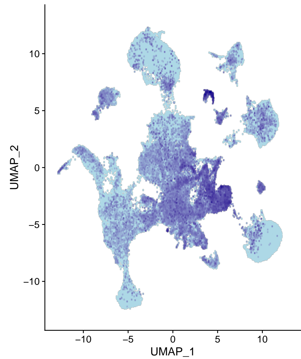
Sphkap
