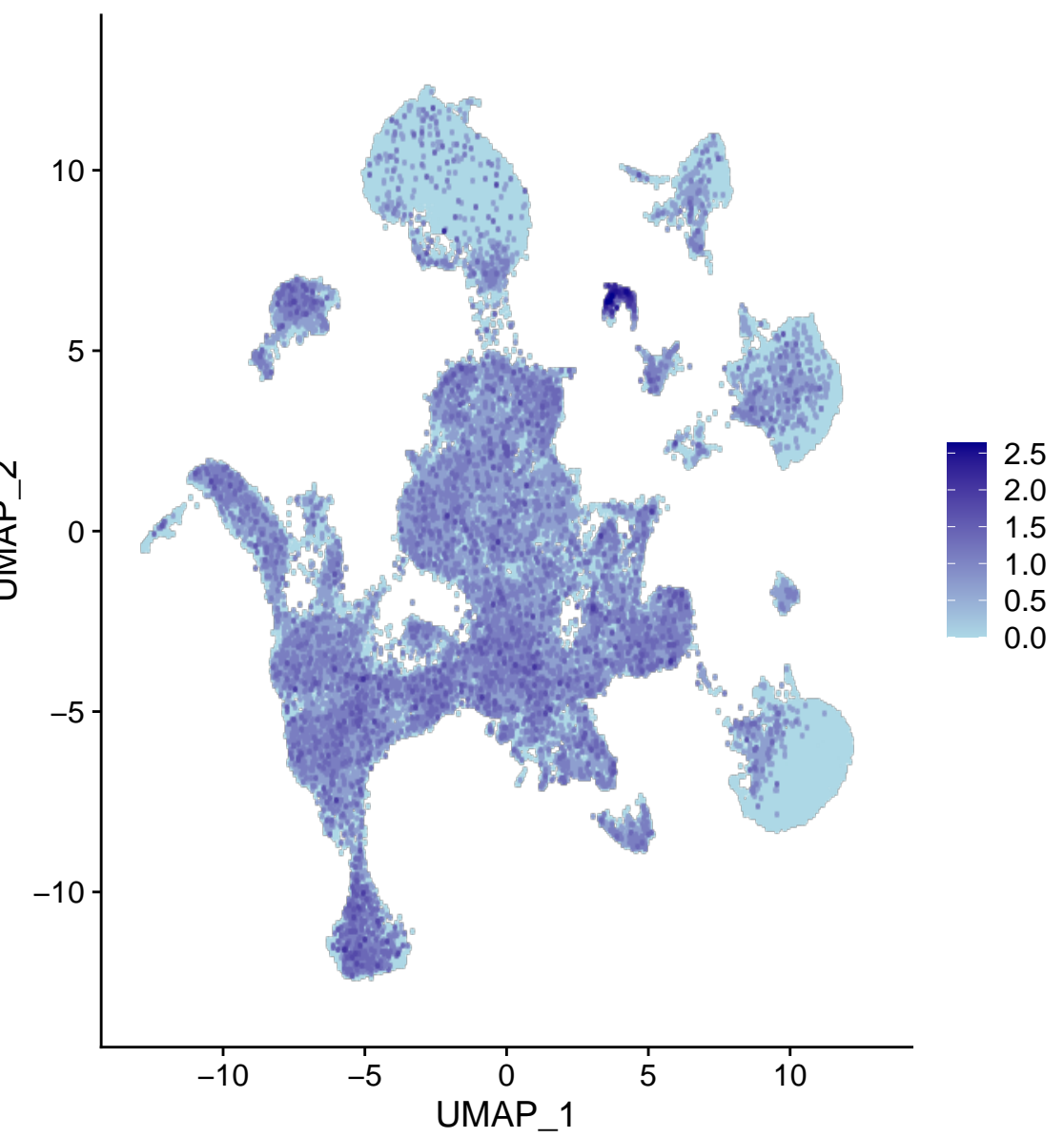
Chrm2
