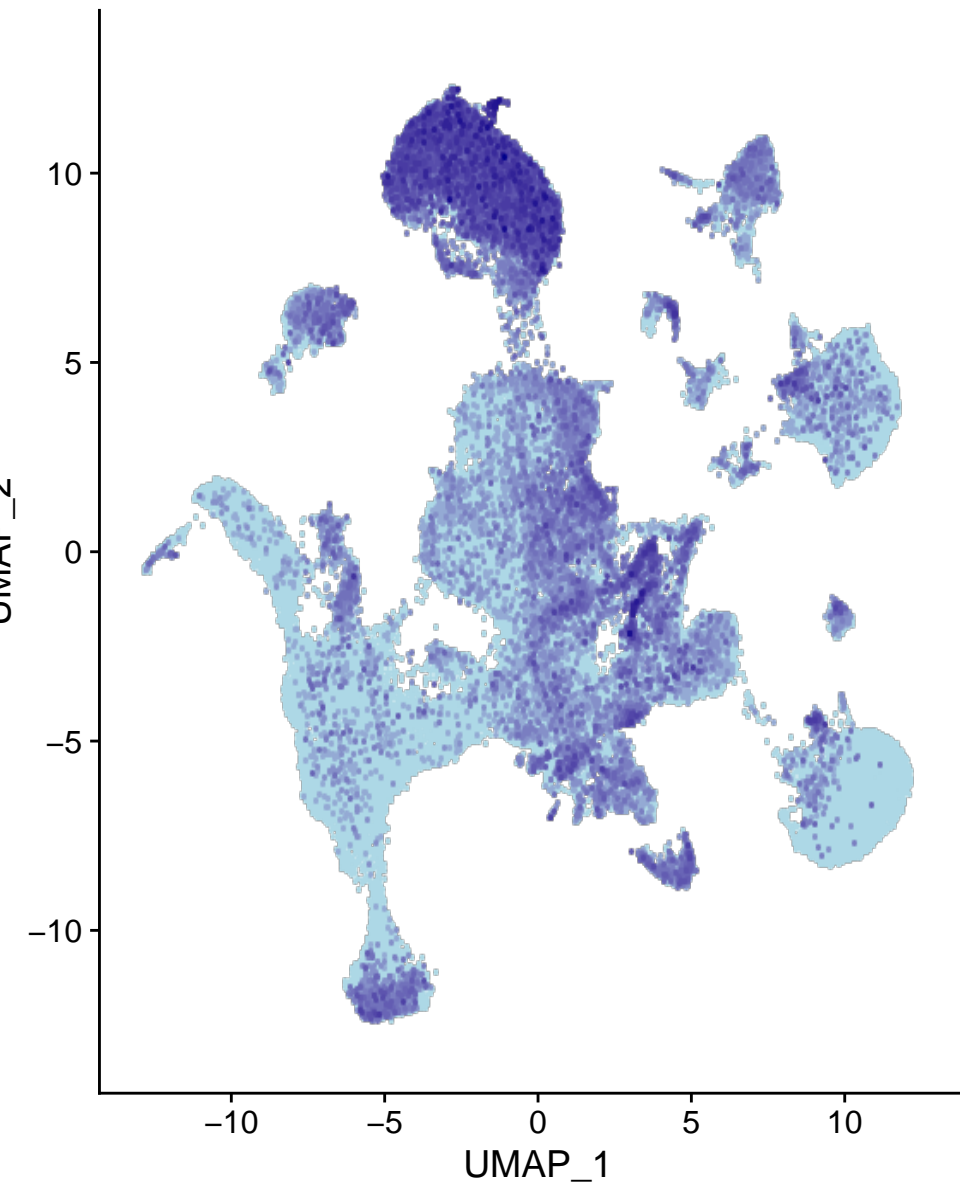
Zfp536
