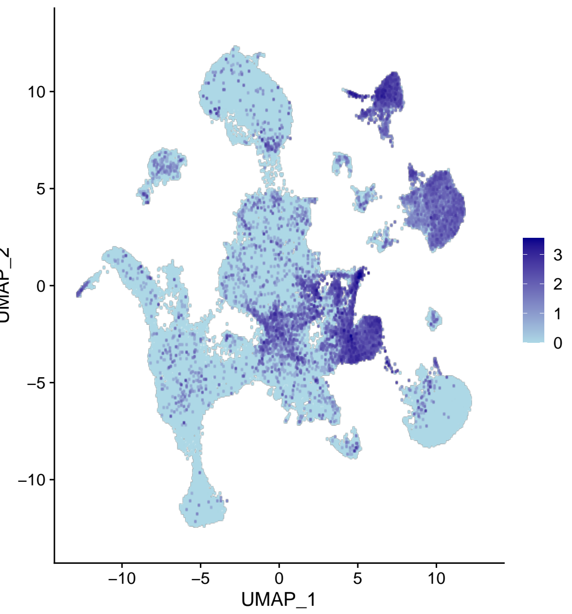
ErbB4
