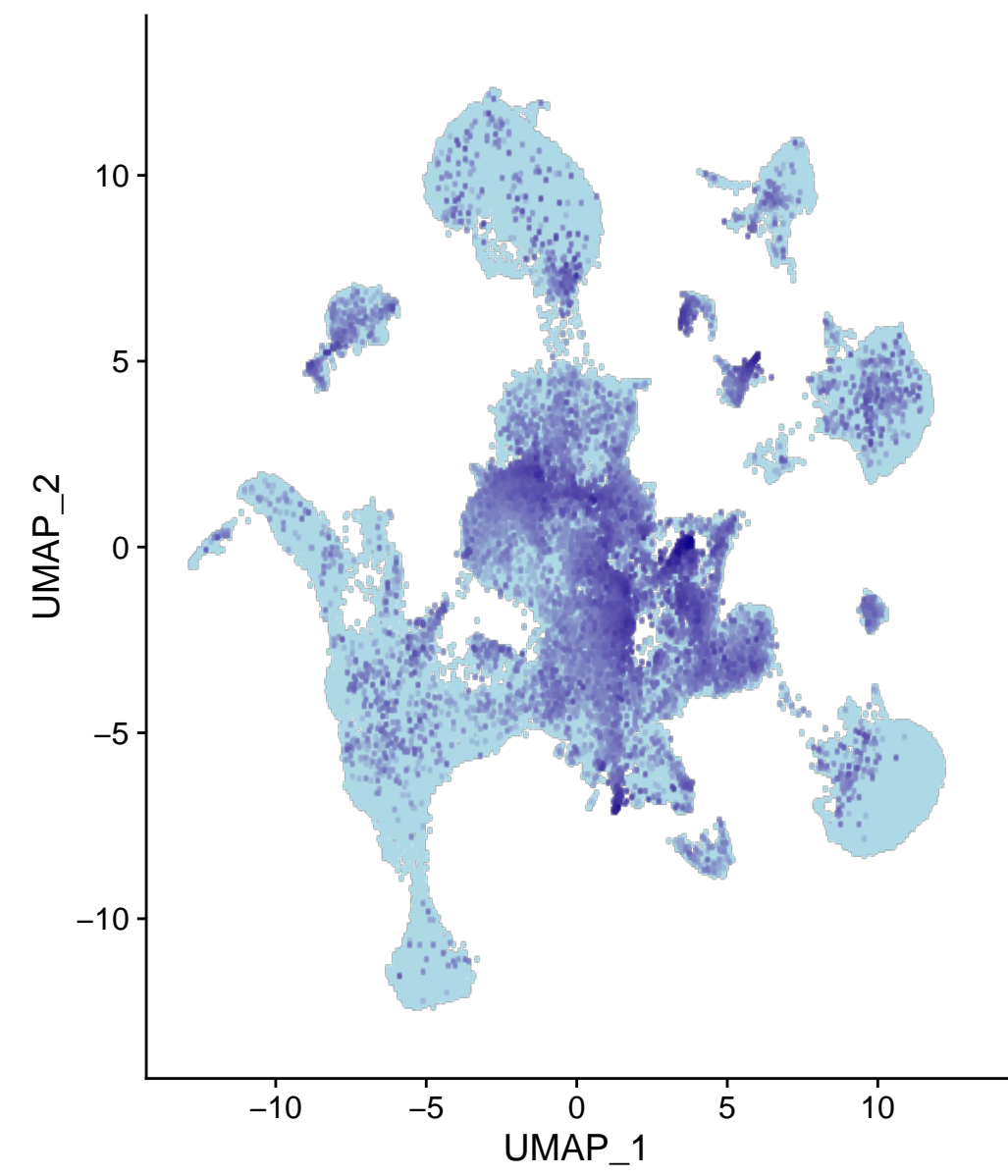
Kcnc2
