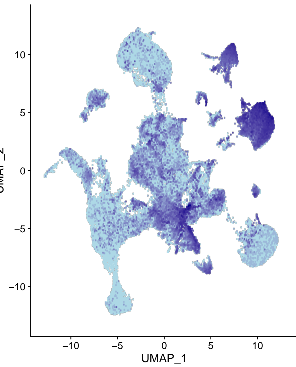
Htr2c
