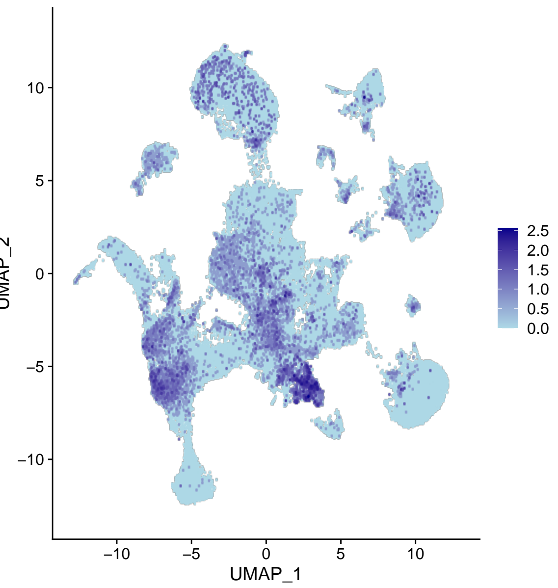
Rmst
