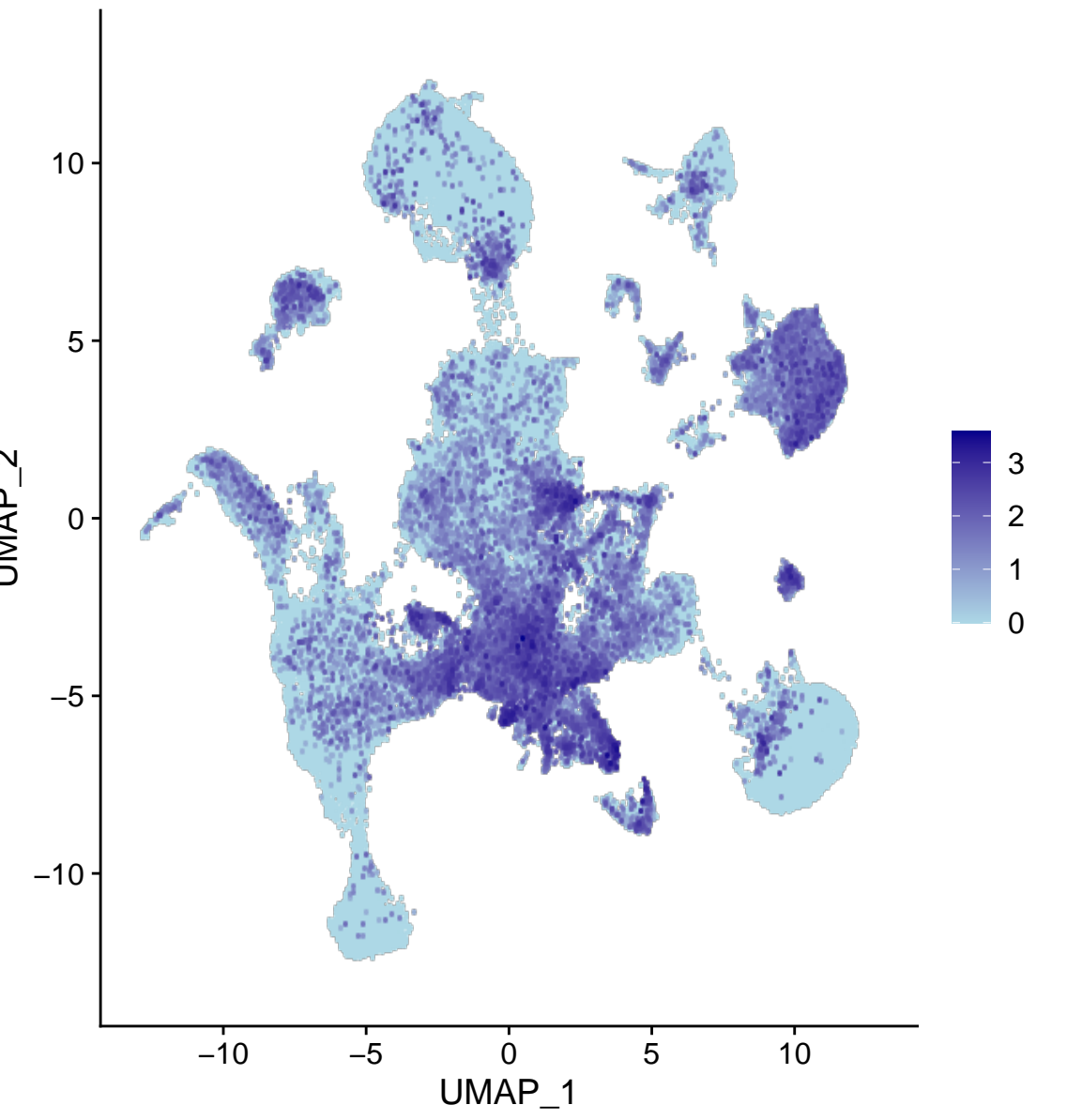
Shisa6
