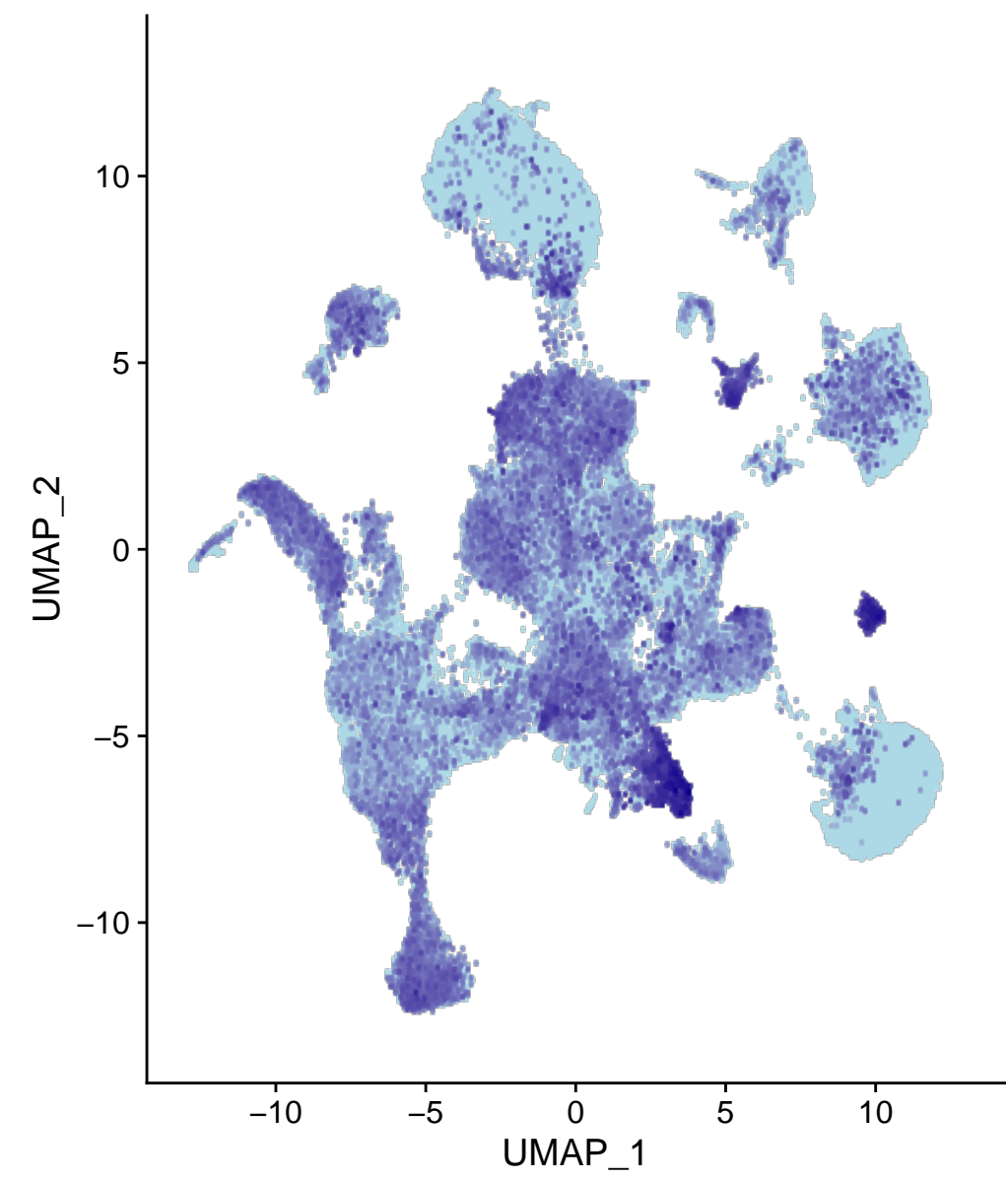
Tafa1
