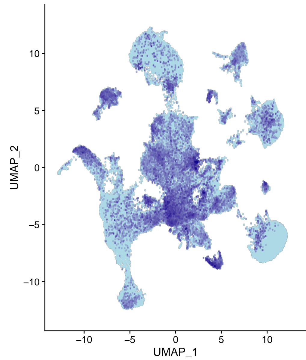
Ncald
