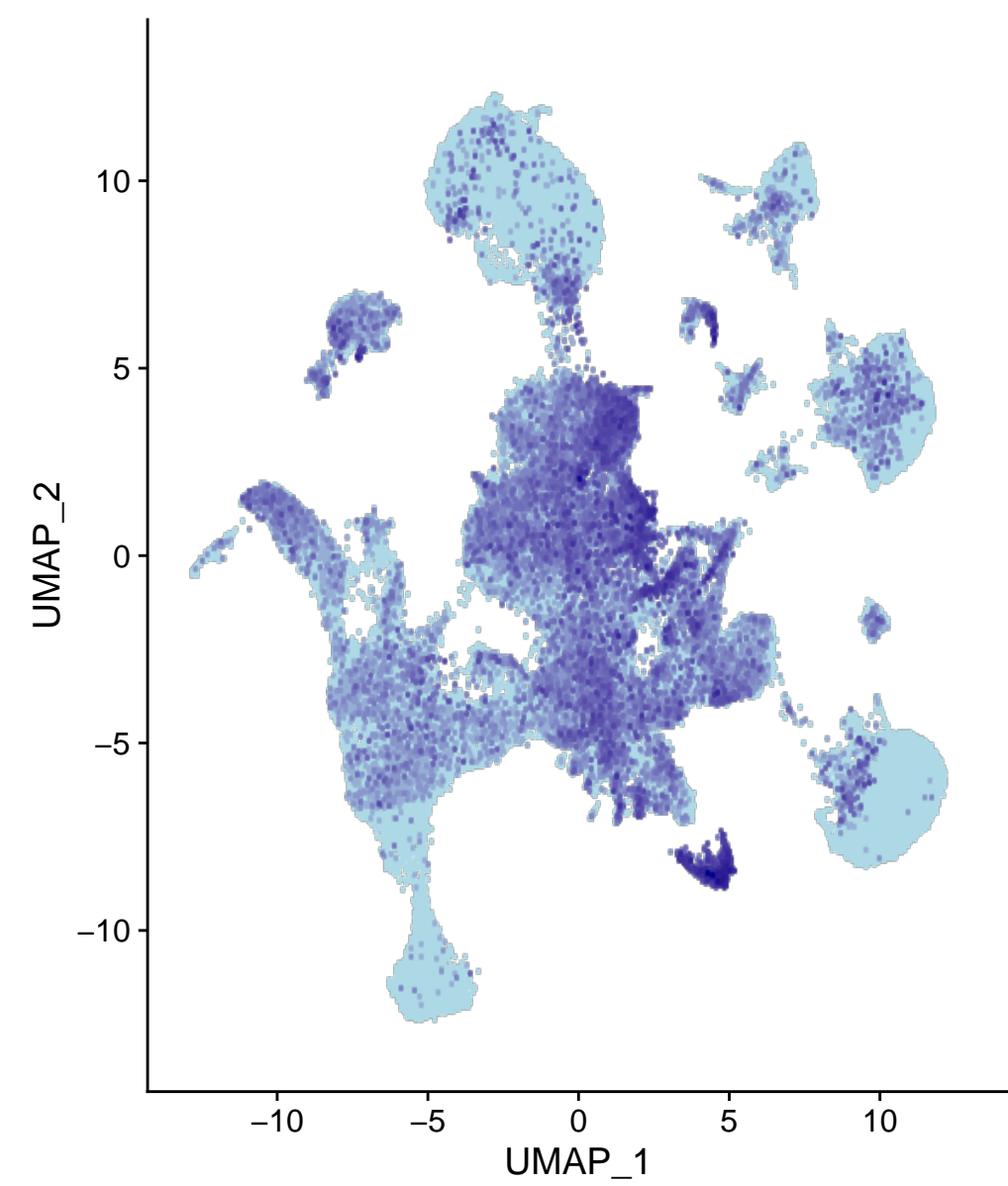
Cadps2
