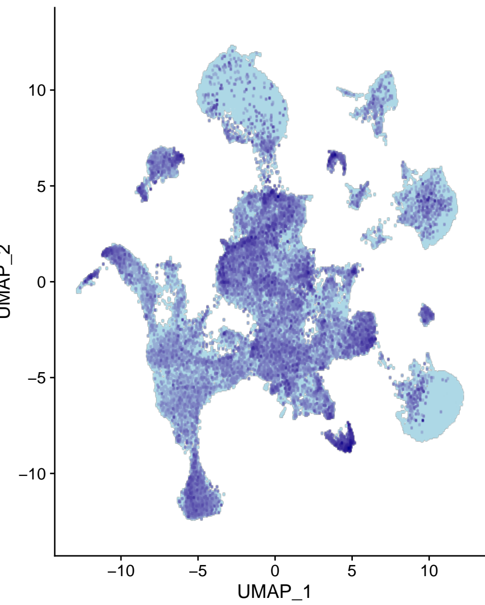
Atp2b4
