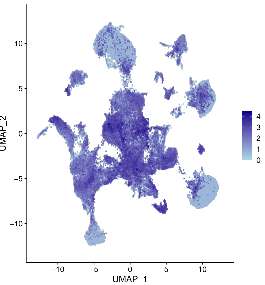
Man1a
