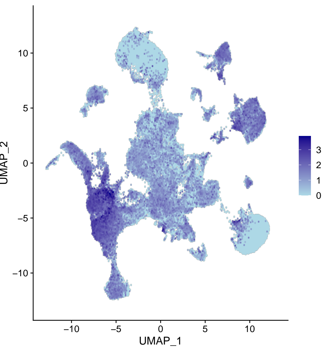
Unc13c
