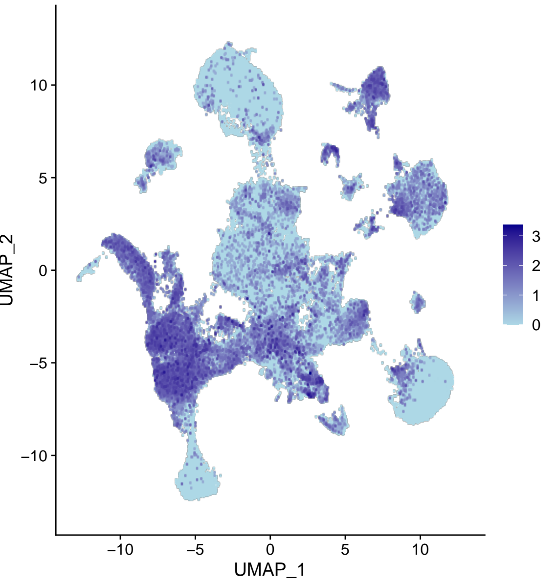
Camk4
