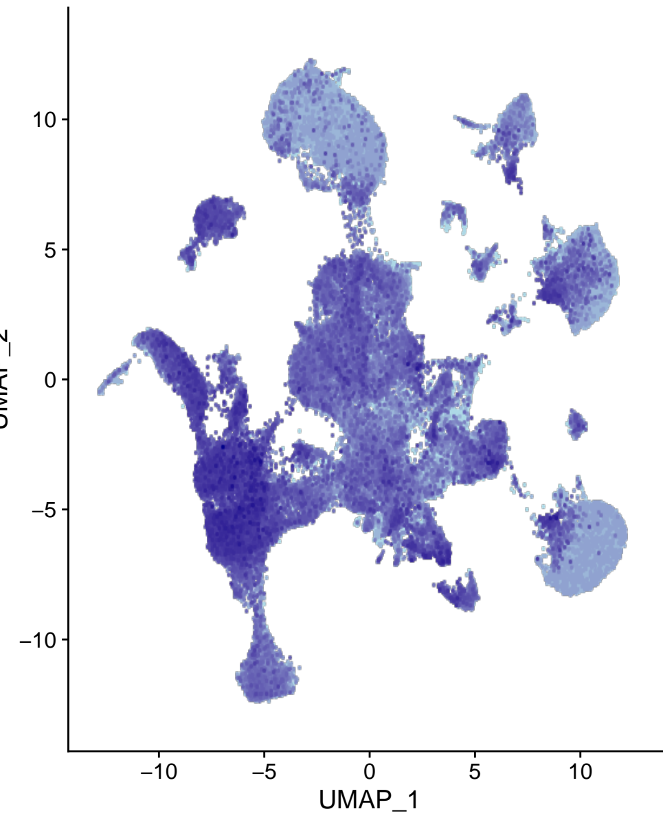
Penk
