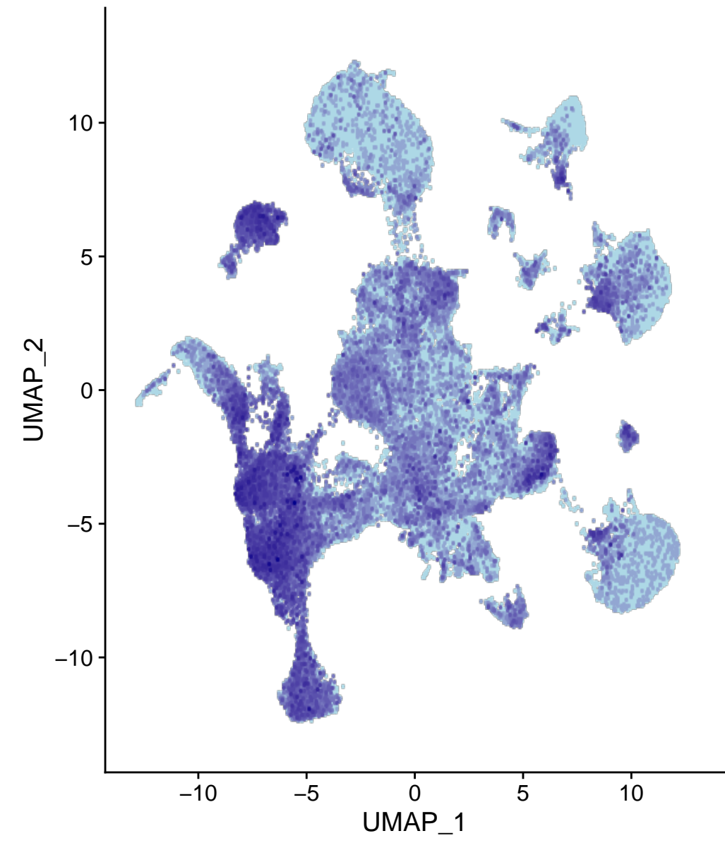
Foxp1
