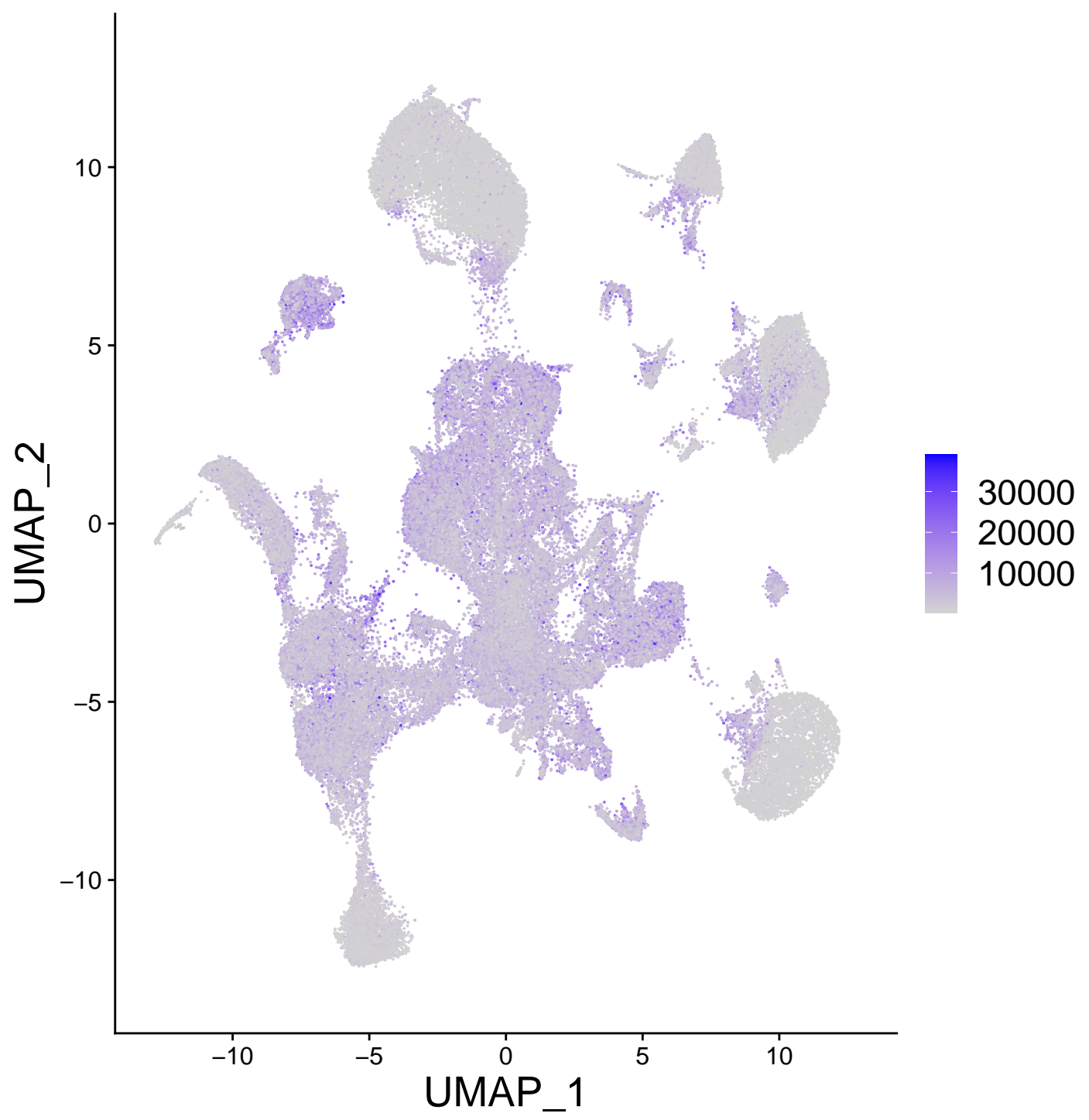
nCount_RNA
