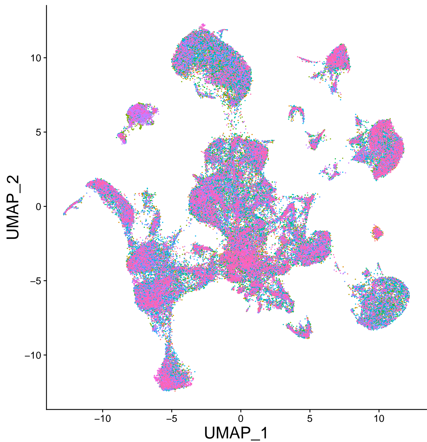
percent.mt
