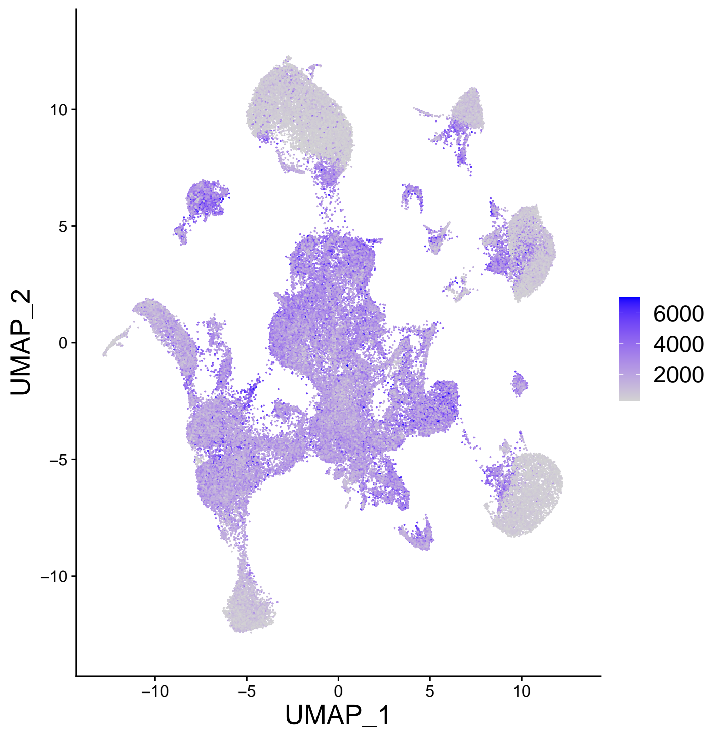
nFeature_RNA
