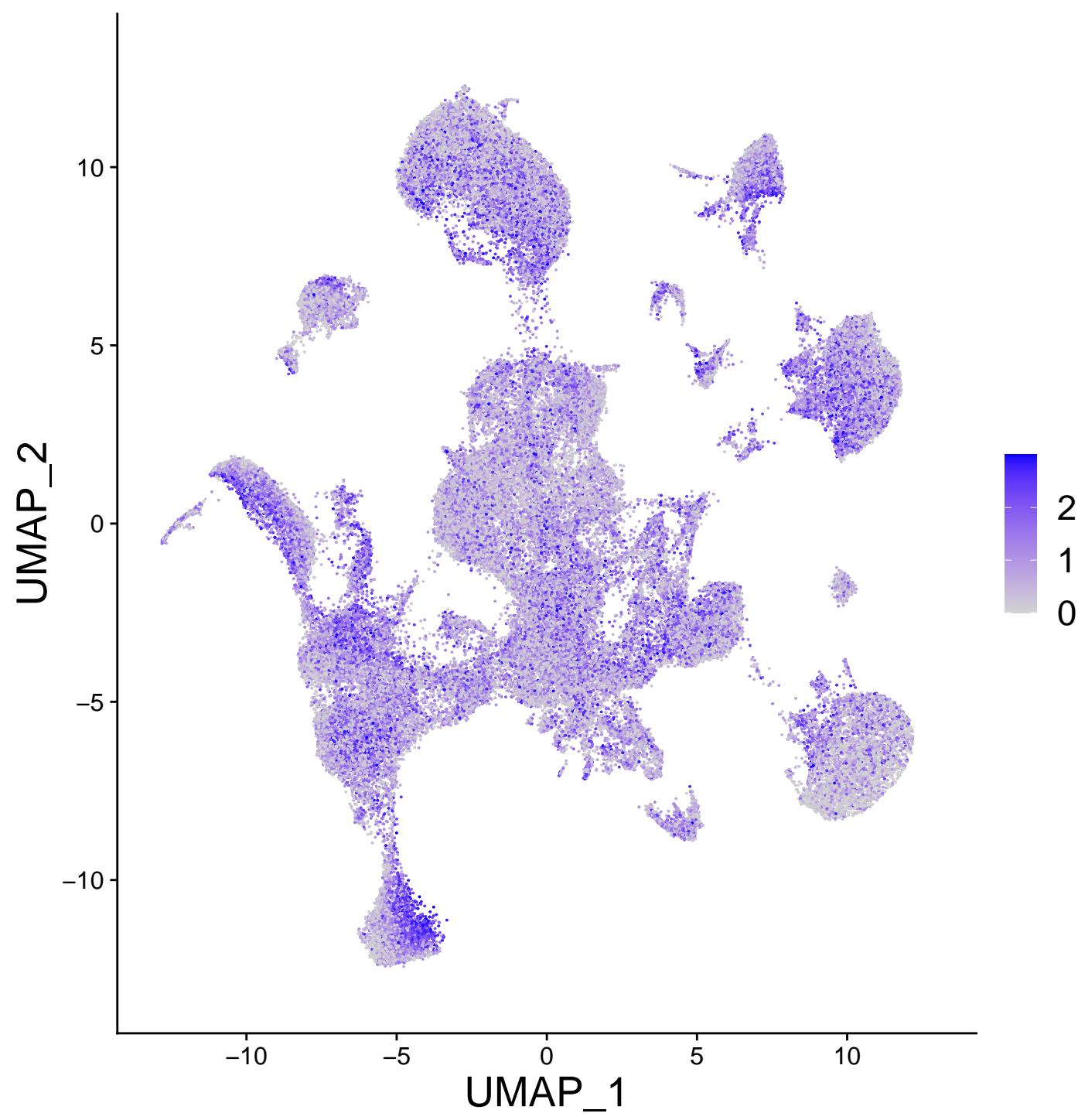
percent.mt
