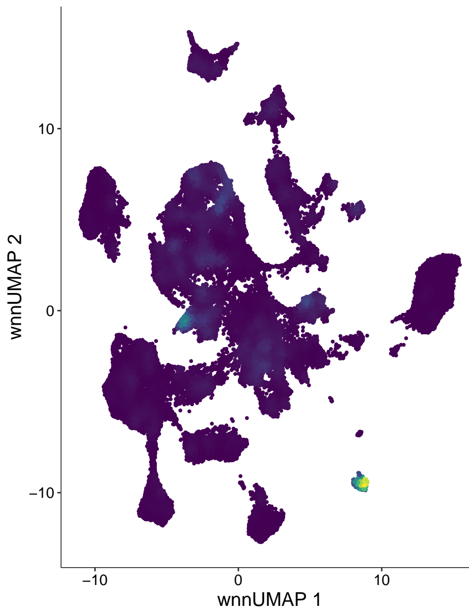
chr3-109917827-109918326
