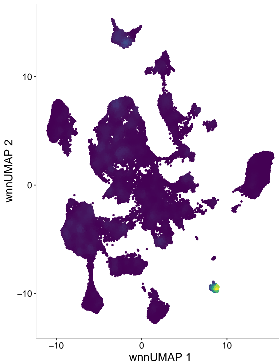
chr12-70157582-70158081
