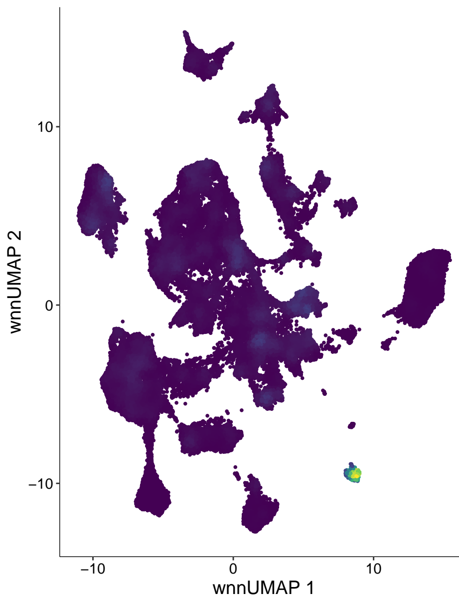
chr12-100123037-100123536
