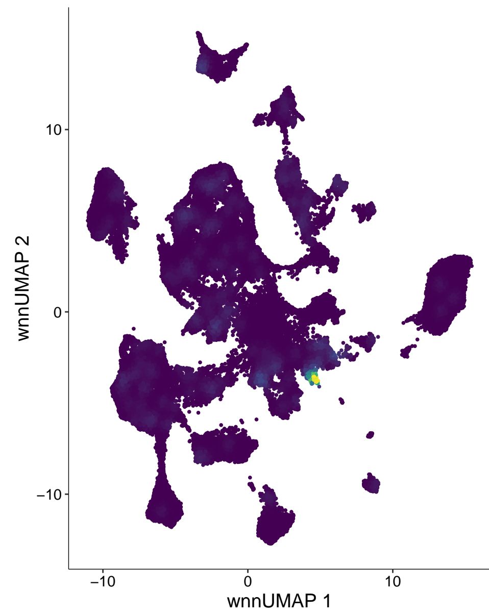
chr11-91056968-91057467
