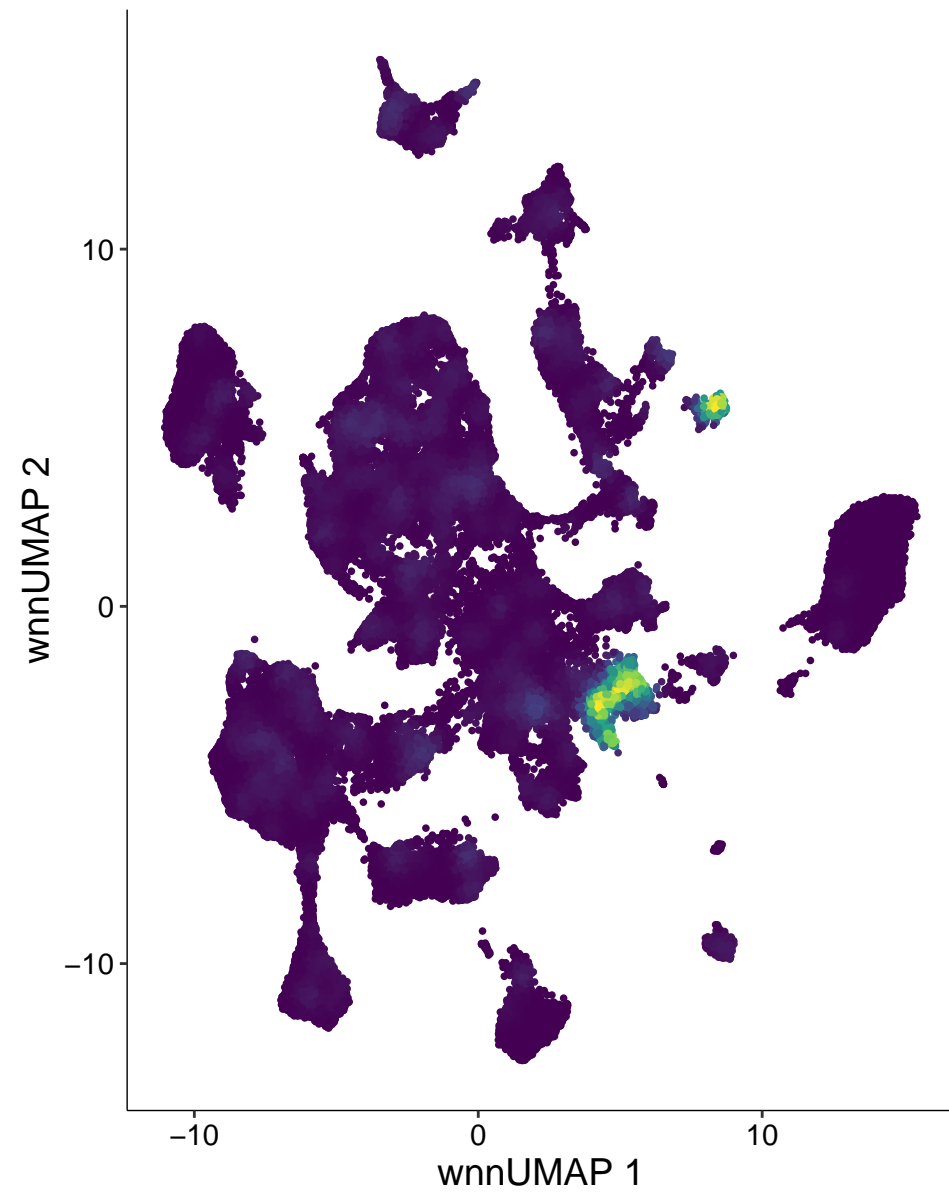
chr1-45425862-45426361
