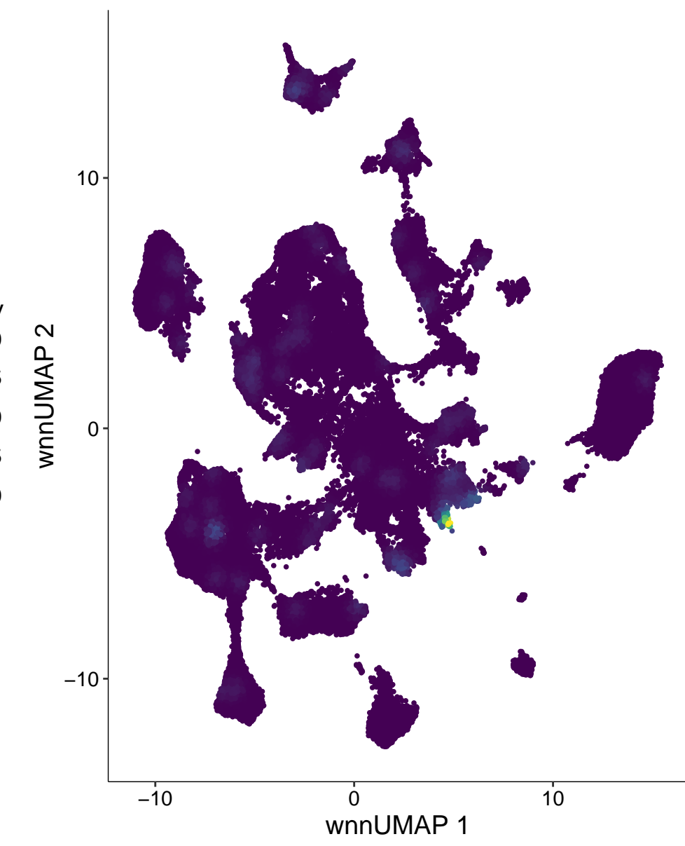
chr11-91034512-91035011
