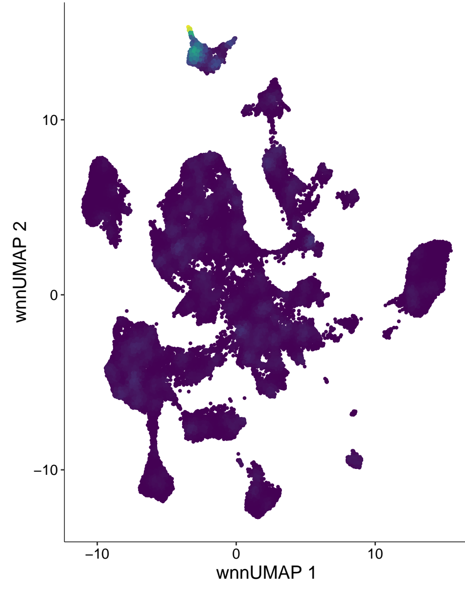
chr7-123823807-123824306
