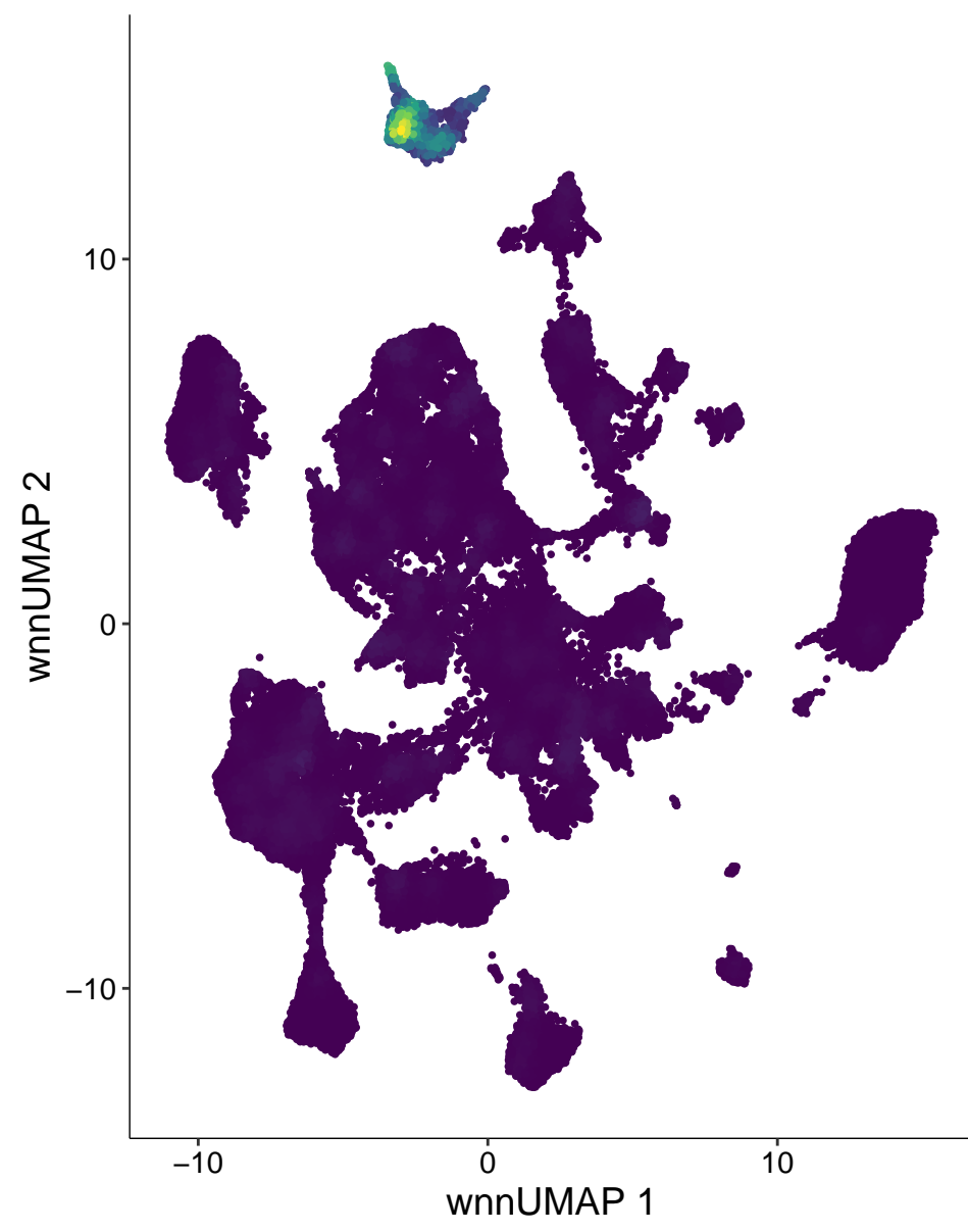
chr7-81730967-81731466
