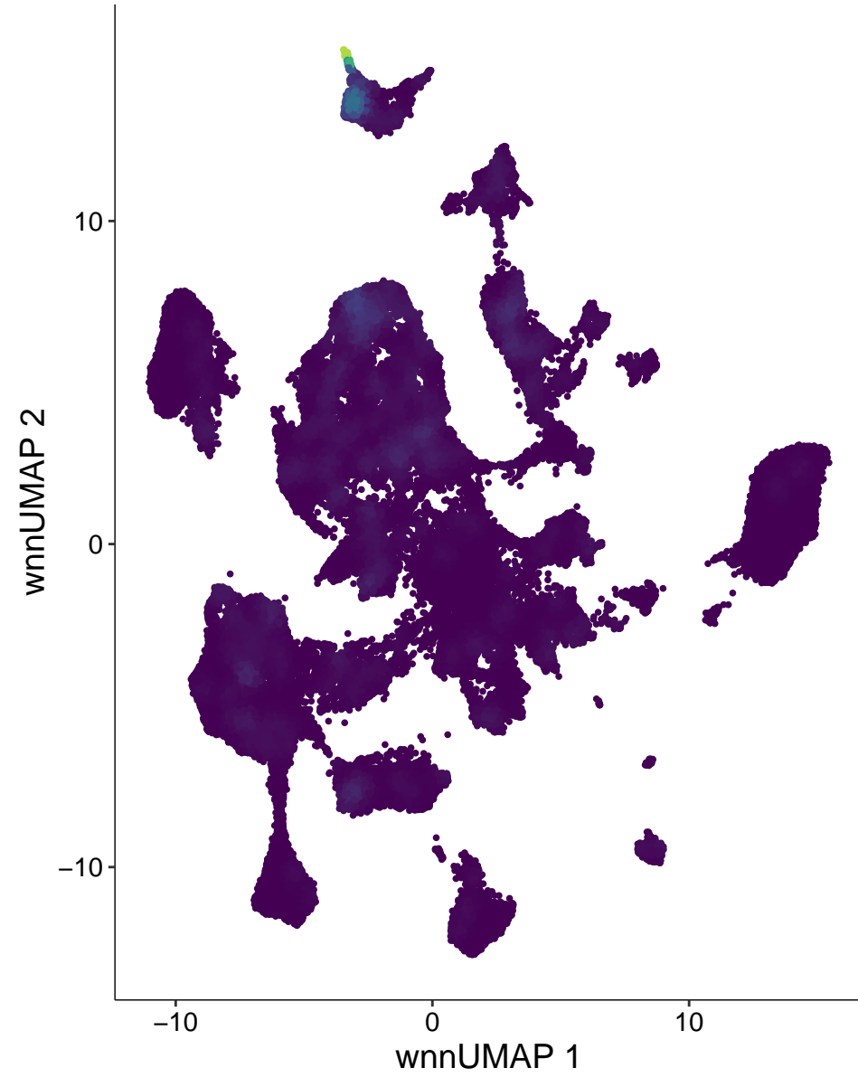
chr19-35418256-35418755
