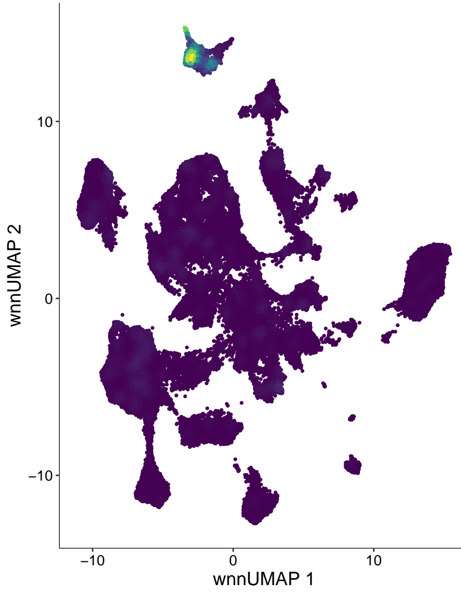
chr5-97134772-97135271
