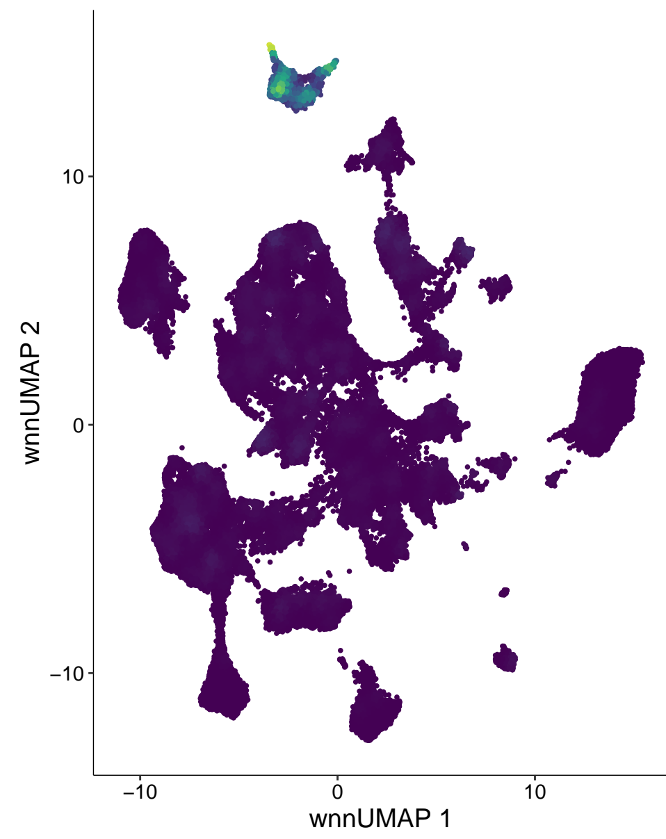
chr19-22796871-22797370
