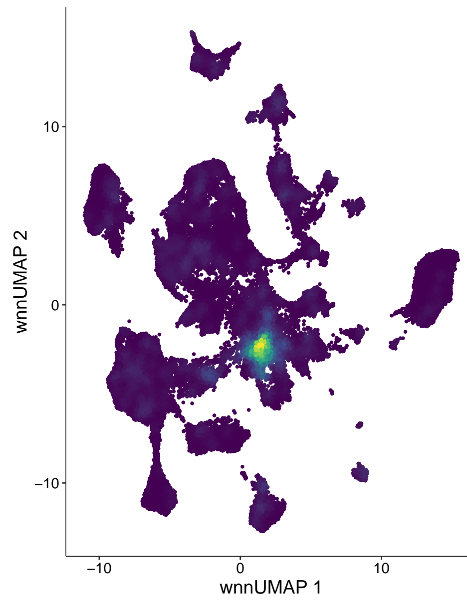
chr5-5871186-5871685
