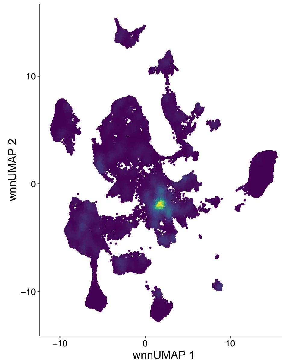
chr2-149661010-149661509
