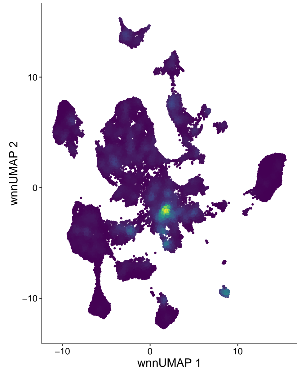
chr12-11221390-11221889
