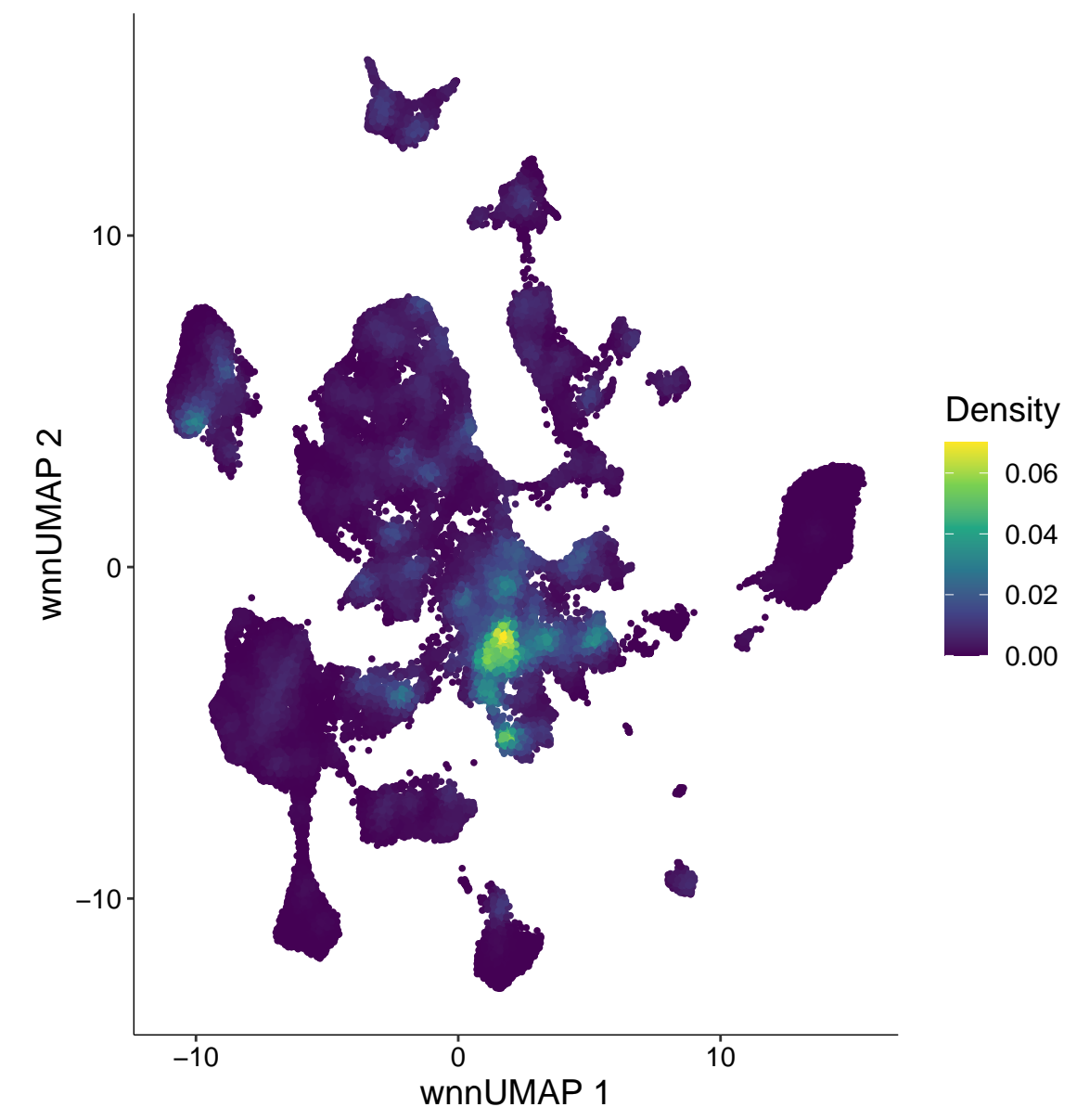
chr10-18181906-18182405
