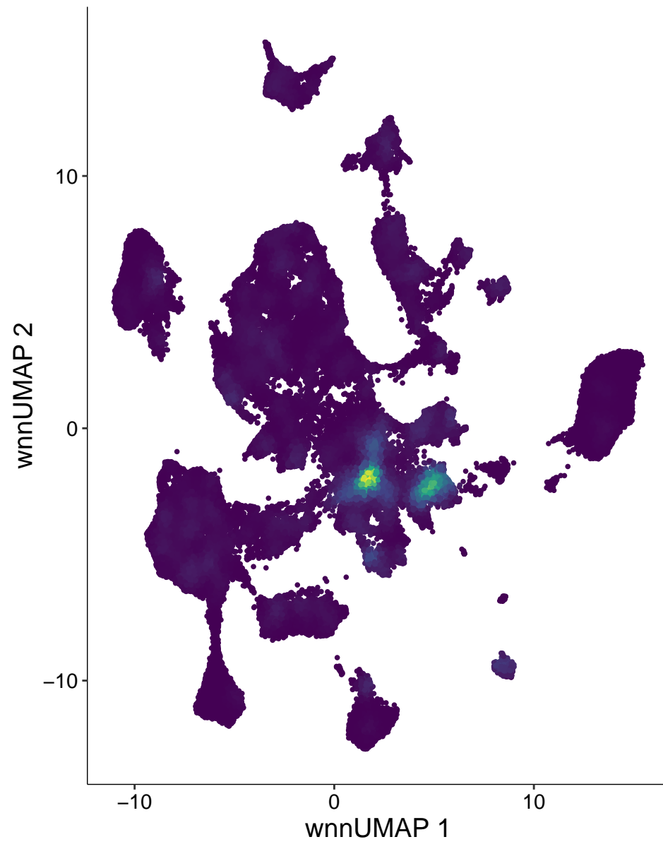
chr1-23359401-23359900
