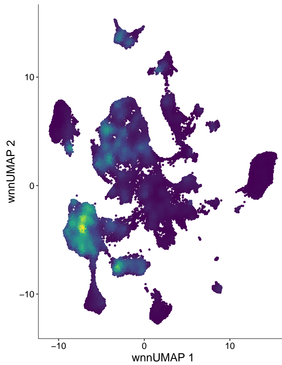
chr2-152101663-152102162
