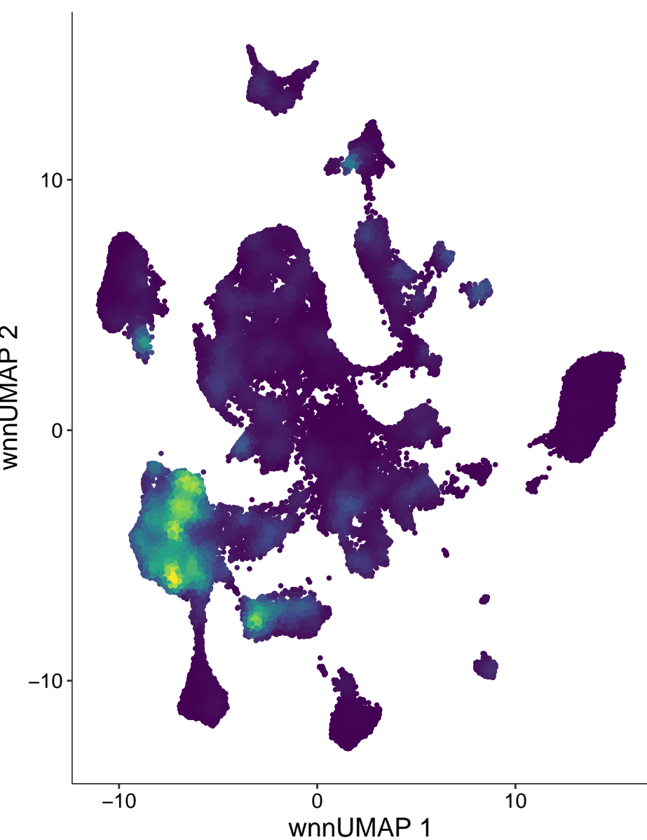
chr15-38165799-38166298
