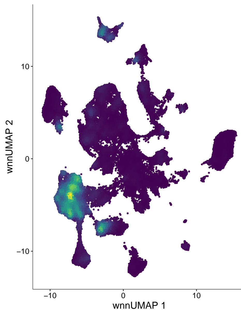
chr18-15078455-15078954
